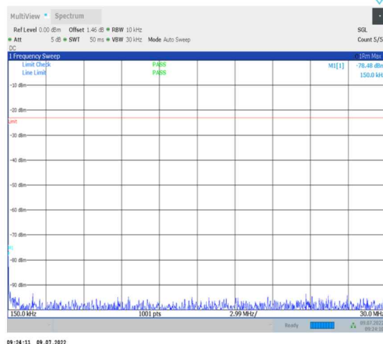
1-N26-824-849-PC3-15-20-H-1-DFT-PI2BPSK- Inner_1RB_Left-1@1-0.15-30-Ant0--78.48--33-PASS
