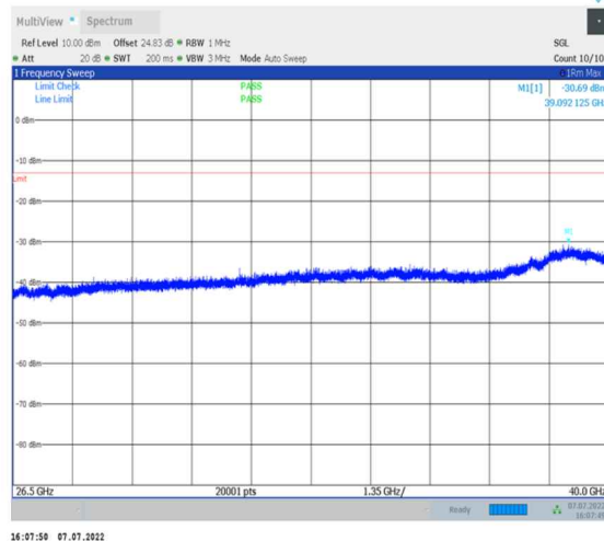
1-N26-824-849-PC3-15-20-M-1-DFT-PI2BPSK- Inner_1RB_Left-1@1-26500-40000-Ant0--30.69--13- PASS
