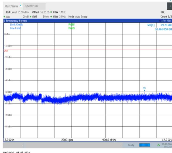
1-N26-824-849-PC3-15-20-L-1-DFT-PI2BPSK- Inner_1RB_Left-1@1-3000-12000-Ant0--49.70--13- PASS
