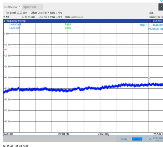
1-N26-824-849-PC3-15-20-M-1-DFT-PI2BPSK- Inner_1RB_Left-1@1-6000-26500-Ant0--44.16--13- PASS
