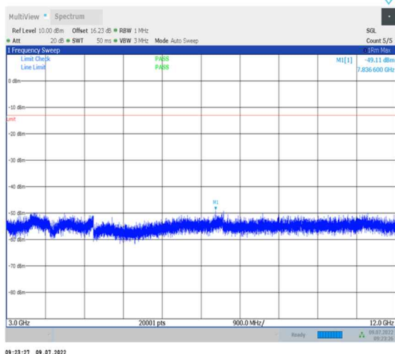
1-N26-824-849-PC3-15-20-M-1-DFT-PI2BPSK- Inner_1RB_Left-1@1-3000-12000-Ant0--49.11--13- PASS
