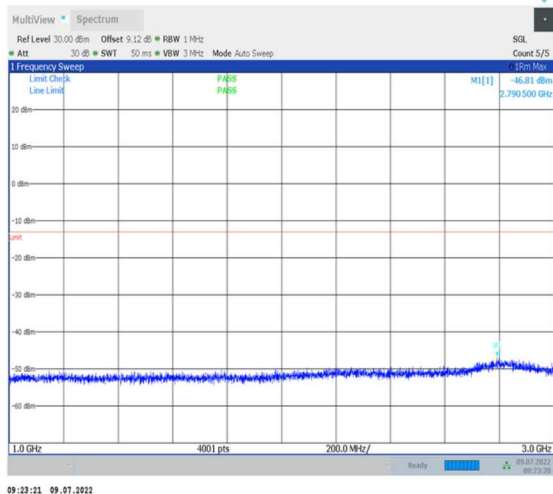
1-N26-824-849-PC3-15-20-M-1-DFT-PI2BPSK- Inner_1RB_Left-1@1-1000-3000-Ant0--46.81--13- PASS
