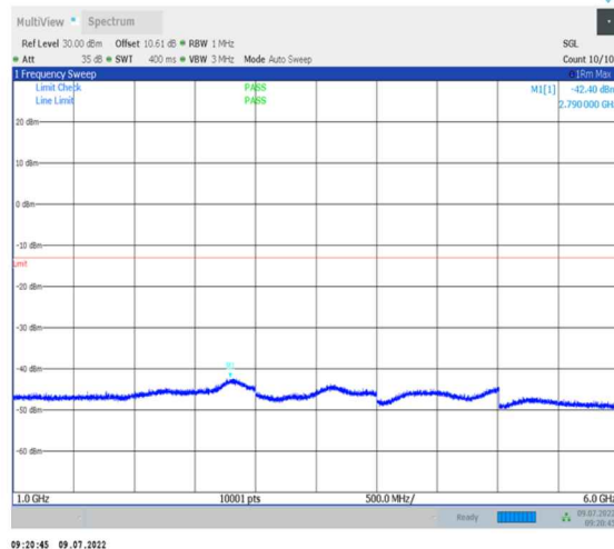
1-N26-824-849-PC3-15-20-M-1-DFT-PI2BPSK- Inner_1RB_Left-1@1-1000-6000-Ant0--42.40--13- PASS
