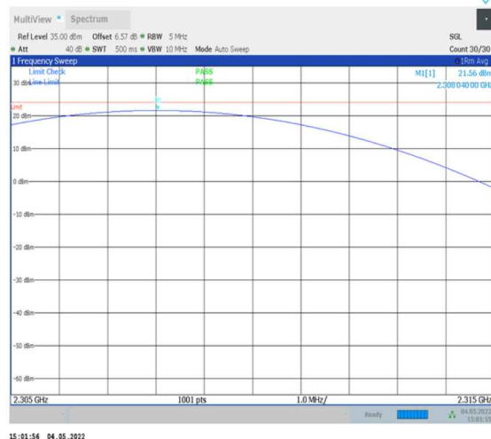
1-N30-PC3-15-5-M-1-DFT-PI2BPSK-Inner_1RB_Left- 1@1-2305-2315-Ant0-21.56-23.98-PASS
