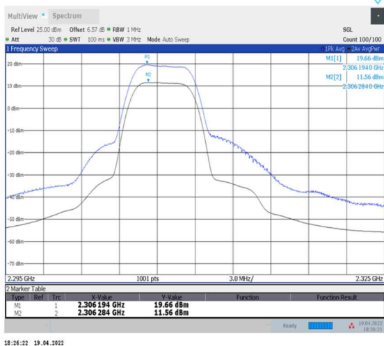
1-N30--15-10-M-1-DFT-256QAM-Outer_Full-24@0- Ant0-8.10-100%-0.00-8.10-PASS-≤13
