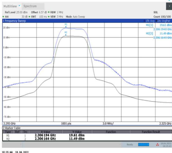
1-N30--15-10-L-1-DFT-256QAM-Outer_Full-24@0- Ant0-8.12-100%-0.00-8.12-PASS-≤13
