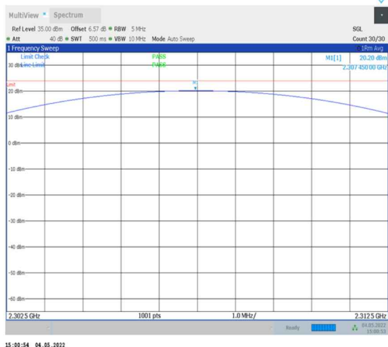
1-N30-PC3-15-5-L-3-DFT-PI2BPSK-Outer_Full- 25@0-2302.5-2312.5-Ant0-20.20-23.98-PASS
