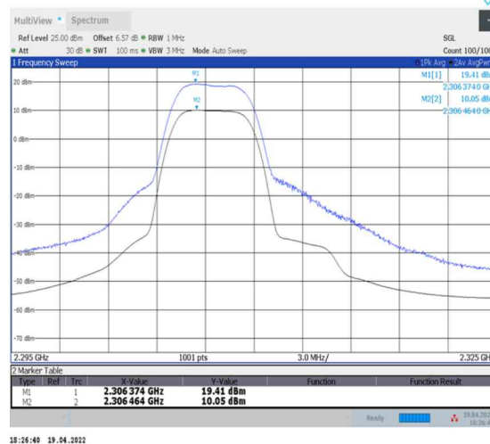
1-N30--15-10-M-2-CP-256QAM-Outer_Full-24@0- Ant0-9.36-100%-0.00-9.36-PASS-≤13
