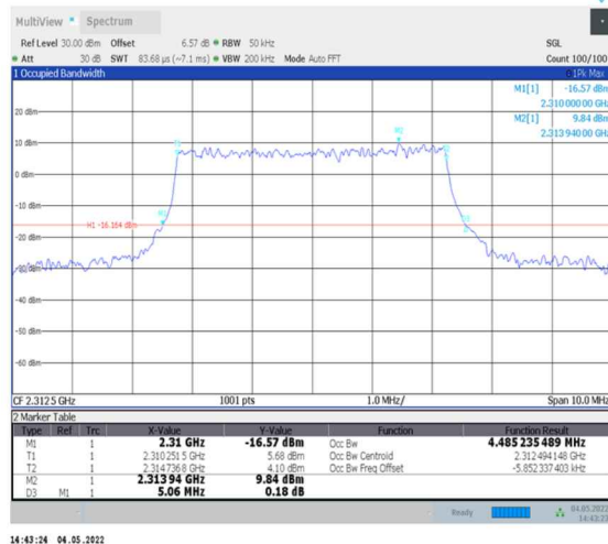
1-N30--15-5-H-8-CP-64QAM-Outer_Full-25@0-Ant0-4.485-5.060-≤5-PASS
