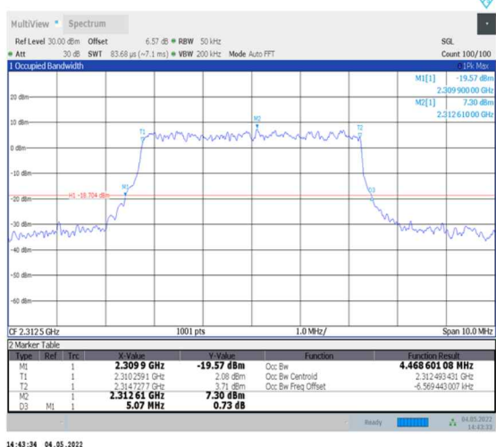
1-N30--15-5-H-9-CP-256QAM-Outer_Full-25@0-Ant0-4.469-5.070-≤5-PASS
