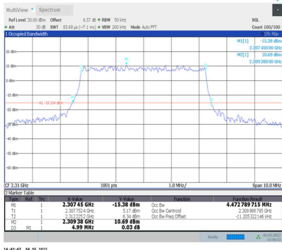
1-N30--15-5-M-4-DFT-64QAM-Outer_Full-25@0- Ant0-4.473-4.990-≤5-PASS
