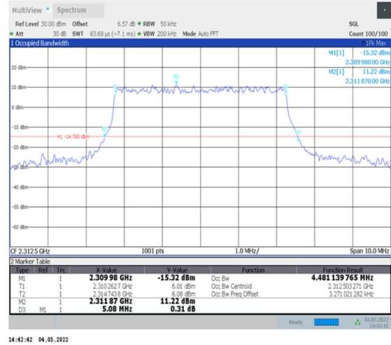
1-N30--15-5-H-4-DFT-64QAM-Outer_Full-25@0-Ant0-4.481-5.080-≤5-PASS
