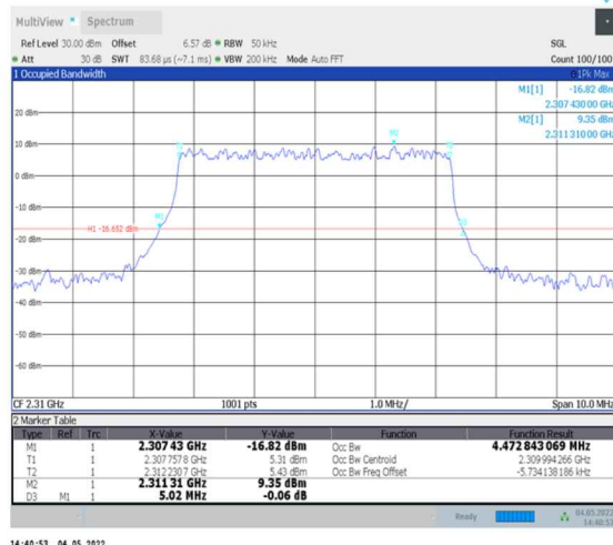
1-N30--15-5-M-5-DFT-256QAM-Outer_Full-25@0- Ant0-4.473-5.020-≤5-PASS
