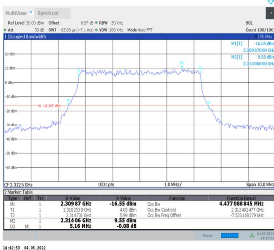
1-N30--15-5-H-5-DFT-256QAM-Outer_Full-25@0-Ant0-4.477-5.160-≤5-PASS
