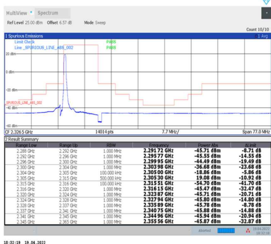
1-N30--30-10-L-4-CP-QPSK-Edge_1RB_Left-1@0-Ant0-PASS-see graph
