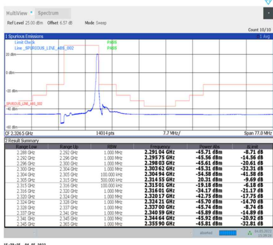
1-N30--15-10-H-5-CP-QPSK-Edge_1RB_Right-1@51-Ant0-PASS-see graph
