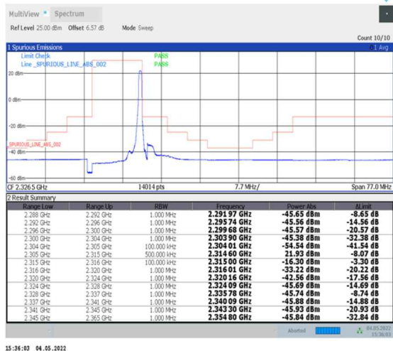
1-N30--15-10-H-2-DFT-PI2BPSK-Edge_1RB_Right-1@51-Ant0-PASS-see graph
