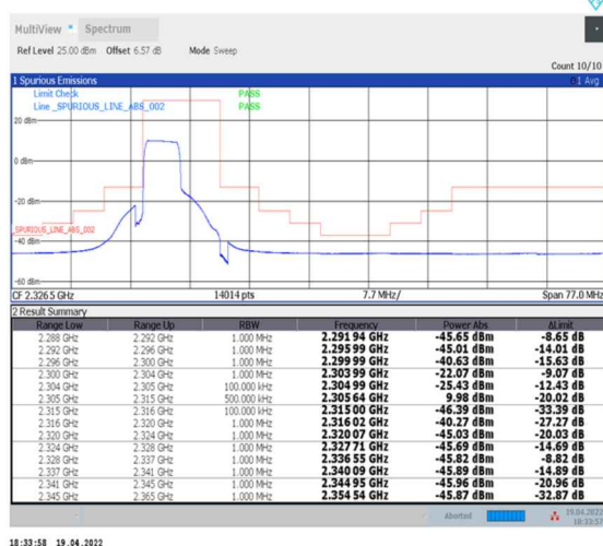
1-N30--30-10-L-6-CP-QPSK-Outer_Full-24@0-Ant0-PASS-see graph
