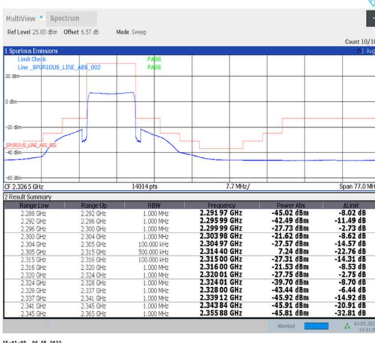
1-N30--15-10-H-6-CP-QPSK-Outer_Full-52@0-Ant0-PASS-see graph
