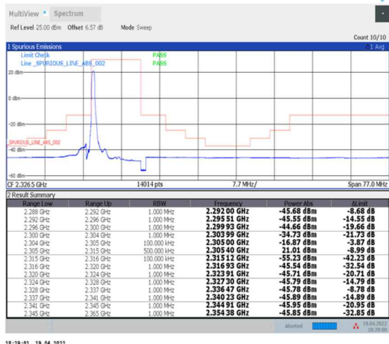
1-N30--30-10-L-1-DFT-PI2BPSK-Edge_1RB_Left-1@0-Ant0-PASS-see graph
