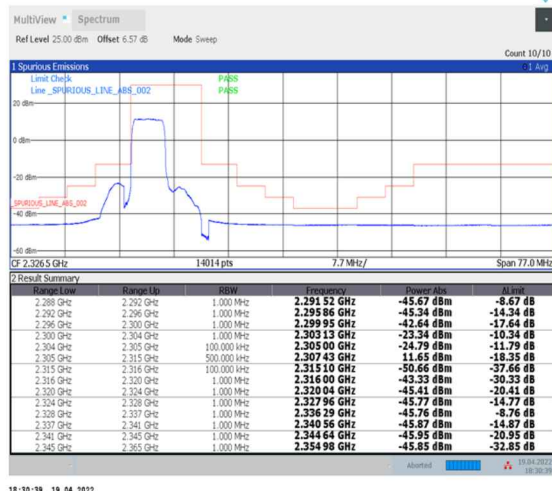
1-N30--30-10-L-3-DFT-PI2BPSK-Outer_Full-24@0-Ant0-PASS-see graph
