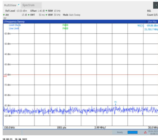
1-N30--30-10-L-1-DFT-PI2BPSK-Inner_1RB_Left- 1@1-0.15-30-Ant0--89.86--60-PASS
