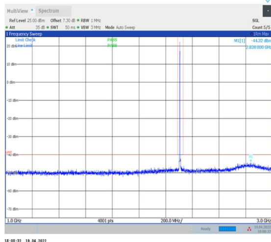
1-N30--15-10-L-1-DFT-PI2BPSK-Inner_1RB_Left- 1@1-1000-3000-Ant0--44.32--40-PASS
