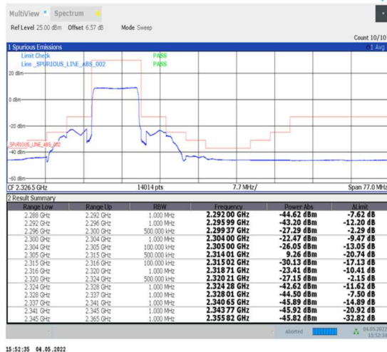
1-N30--15-10-H-3-DFT-PI2BPSK-Outer_Full-50@0-Ant0-PASS-see graph
