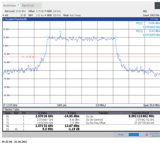
1-N38--30-10-L-3-DFT-16QAM-Outer_Full-24@0- Ant0-8.592-9.500-≤10-PASS
