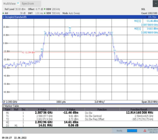
1-N38--30-15-M-1-DFT-QPSK-Outer_Full-36@0-Ant0-12.914-14.010-≤15-PASS
