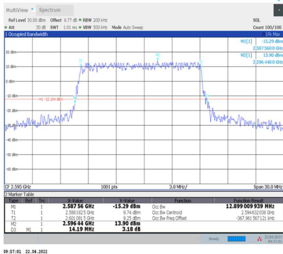
1-N38--30-15-M-3-DFT-16QAM-Outer_Full-36@0-Ant0-12.899-14.190-≤15-PASS
