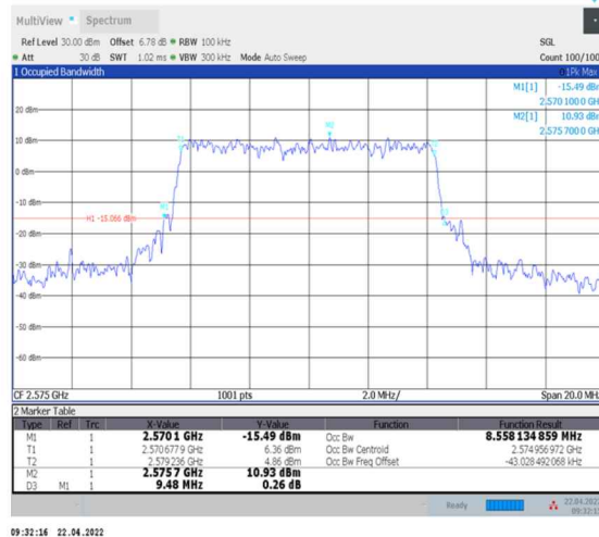
1-N38--30-10-L-4-DFT-64QAM-Outer_Full-24@0- Ant0-8.558-9.480-≤10-PASS
