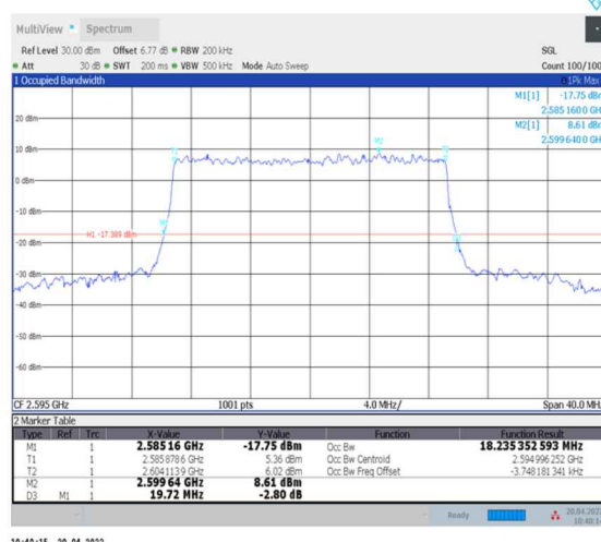
1-N38--30-20-M-9-CP-256QAM-Outer_Full-51@0-Ant0-18.235-19.720-≤20-PASS
