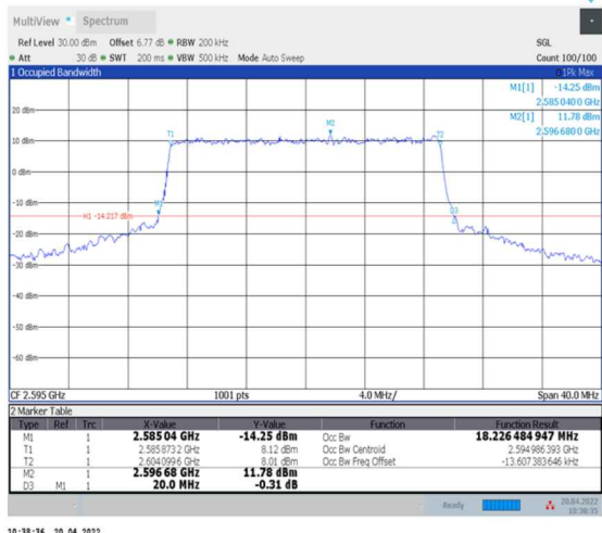
1-N38--30-20-M-6-CP-QPSK-Outer_Full-51@0-Ant0-18.226-20.000-≤20-PASS
