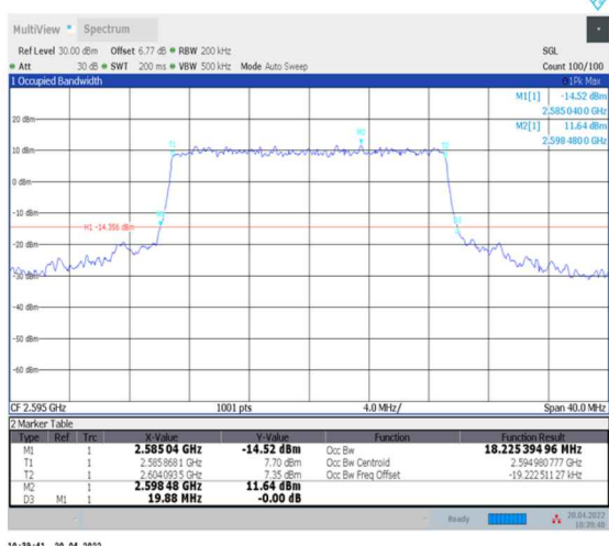
1-N38--30-20-M-8-CP-64QAM-Outer_Full-51@0-Ant0-18.225-19.880-≤20-PASS
