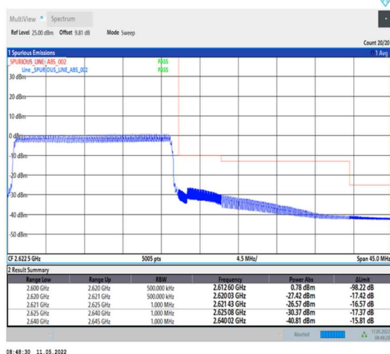
1-N38-PC2-30-20-H-6-CP-QPSK-Outer_Full-51@0-Ant0-PASS-see graph
