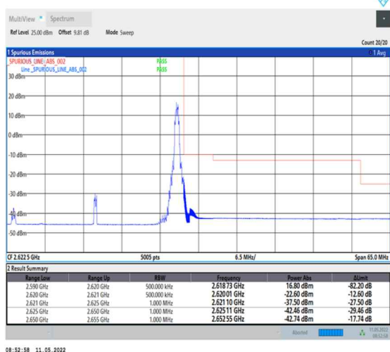
1-N38-PC2-30-30-H-5-CP-QPSK-Edge_1RB_Right-1@77-Ant0-PASS-see graph
