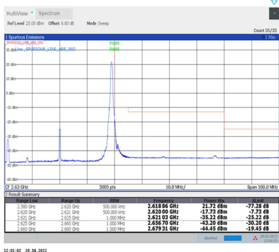
1-N38--30-40-H-5-CP-QPSK-Edge_1RB_Right-1@105-Ant0-PASS-see graph
