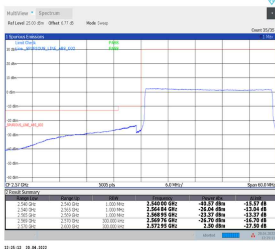
1-N38--30-30-L-6-CP-QPSK-Outer_Full-78@0-Ant0-PASS-see graph
