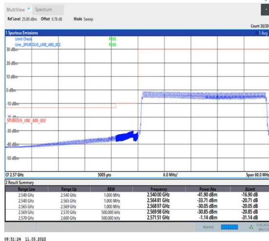
1-N38-PC2-30-30-L-6-CP-QPSK-Outer_Full-78@0-Ant0-PASS-see graph
