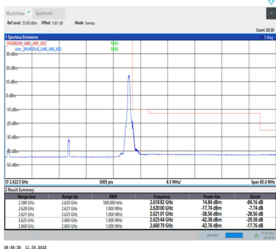
1-N38-PC2-30-40-H-5-CP-QPSK-Edge_1RB_Right-1@105-Ant0-PASS-see graph
