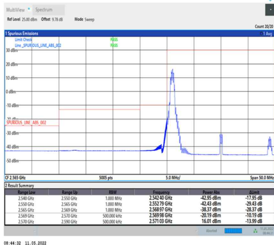
1-N38-PC2-30-20-L-4-CP-QPSK-Edge_1RB_Left-1@0-Ant0-PASS-see graph
