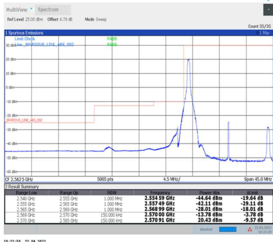
1-N38--30-15-L-1-DFT-PI2BPSK-Edge_1RB_Left-1@0-Ant0-PASS-see graph
