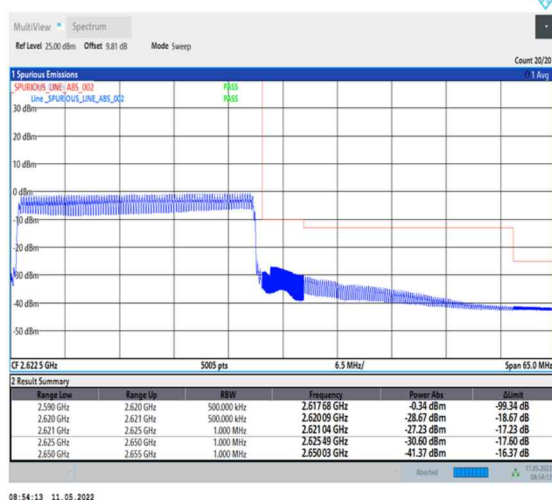
1-N38-PC2-30-30-H-6-CP-QPSK-Outer_Full-78@0-Ant0-PASS-see graph
