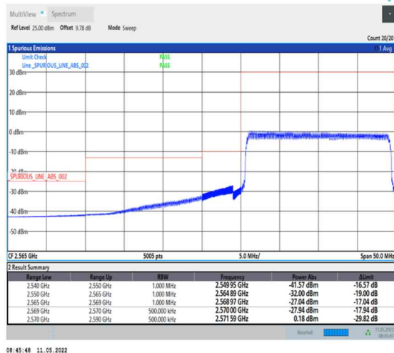
1-N38-PC2-30-20-L-6-CP-QPSK-Outer_Full-51@0-Ant0-PASS-see graph
