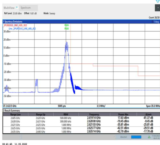
1-N38-PC2-30-15-H-5-CP-QPSK-Edge_1RB_Right-1@37-Ant0-PASS-see graph
