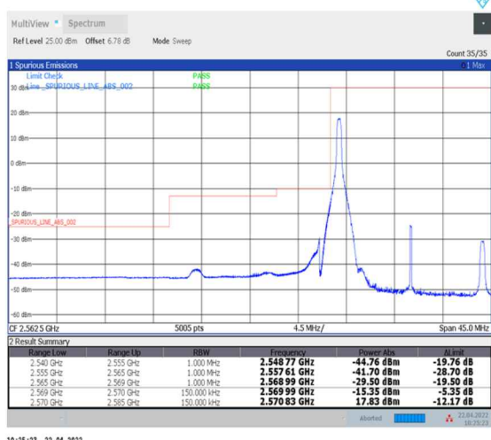
1-N38--30-15-L-4-CP-QPSK-Edge_1RB_Left-1@0-Ant0-PASS-see graph
