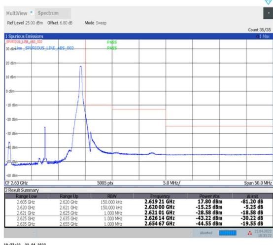
1-N38--30-15-H-5-CP-QPSK-Edge_1RB_Right-1@37-Ant0-PASS-see graph
