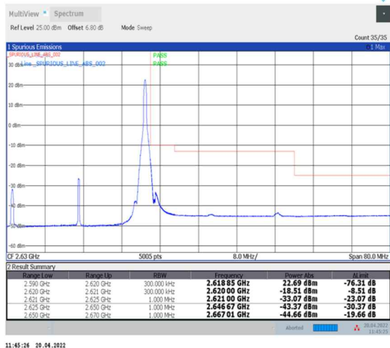
1-N38--30-30-H-2-DFT-PI2BPSK-Edge_1RB_Right-1@77-Ant0-PASS-see graph
