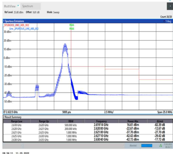
1-N38-PC2-30-10-H-5-CP-QPSK-Edge_1RB_Right-1@23-Ant0-PASS-see graph
