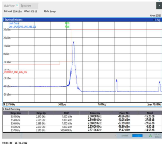
1-N38-PC2-30-40-L-4-CP-QPSK-Edge_1RB_Left-1@0-Ant0-PASS-see graph
