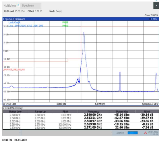
1-N38--30-30-L-1-DFT-PI2BPSK-Edge_1RB_Left-1@0-Ant0-PASS-see graph
