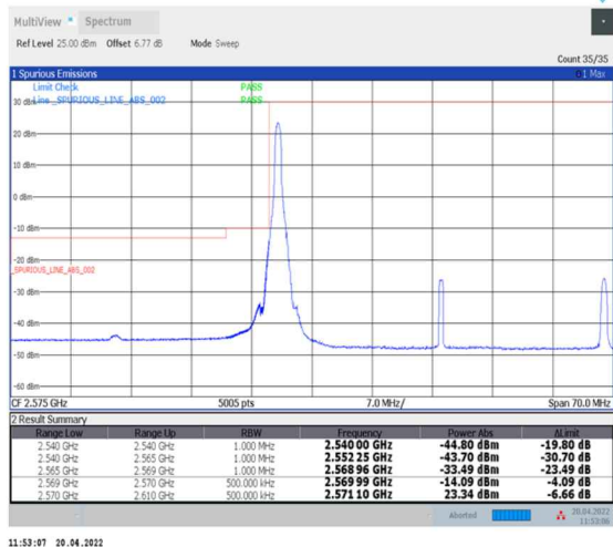
1-N38--30-40-L-1-DFT-PI2BPSK-Edge_1RB_Left-1@0-Ant0-PASS-see graph
