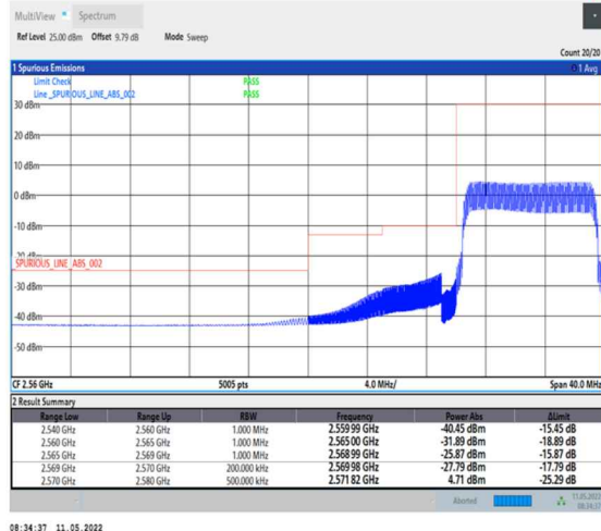
1-N38-PC2-30-10-L-6-CP-QPSK-Outer_Full-24@0-Ant0-PASS-see graph
