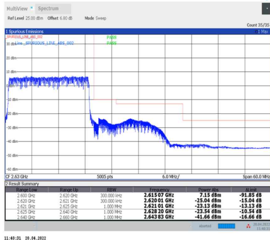
1-N38--30-20-H-3-DFT-PI2BPSK-Outer_Full-50@0-Ant0-PASS-see graph
