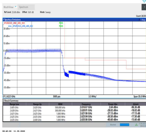
1-N38-PC2-30-15-H-6-CP-QPSK-Outer_Full-38@0-Ant0-PASS-see graph
