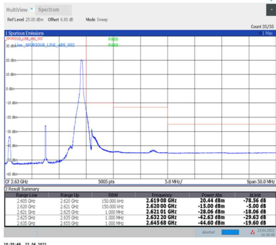
1-N38--30-15-H-2-DFT-PI2BPSK-Edge_1RB_Right-1@37-Ant0-PASS-see graph
