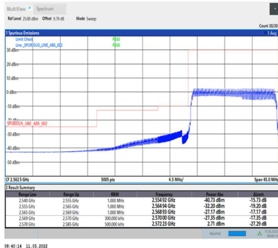
1-N38-PC2-30-15-L-6-CP-QPSK-Outer_Full-38@0-Ant0-PASS-see graph
