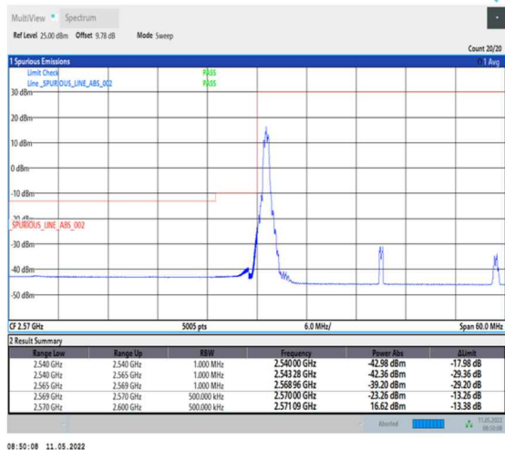
1-N38-PC2-30-30-L-4-CP-QPSK-Edge_1RB_Left-1@0-Ant0-PASS-see graph
