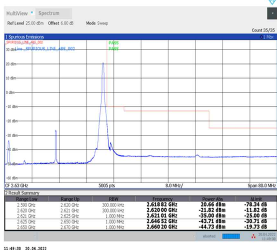
1-N38--30-30-H-5-CP-QPSK-Edge_1RB_Right-1@77-Ant0-PASS-see graph
