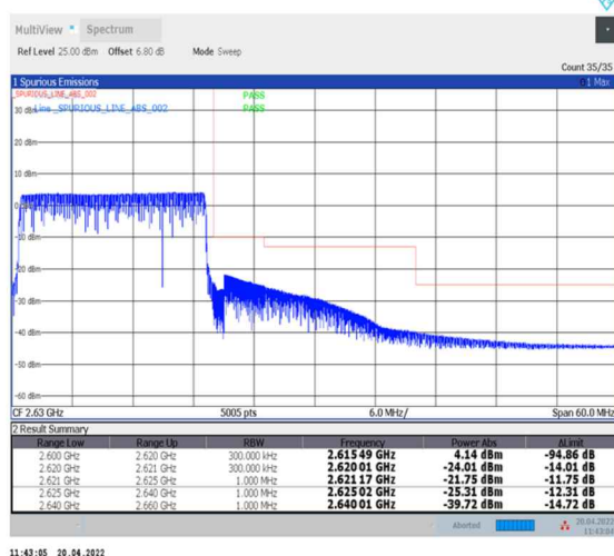
1-N38--30-20-H-6-CP-QPSK-Outer_Full-51@0-Ant0-PASS-see graph
