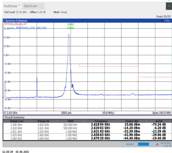
1-N38--30-40-H-2-DFT-PI2BPSK-Edge_1RB_Right-1@105-Ant0-PASS-see graph
