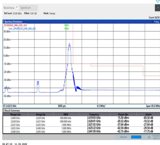
1-N38-PC2-30-20-H-5-CP-QPSK-Edge_1RB_Right-1@50-Ant0-PASS-see graph
