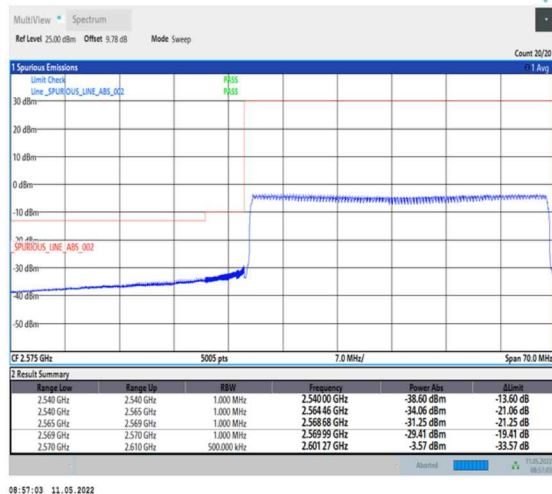
1-N38-PC2-30-40-L-6-CP-QPSK-Outer_Full-106@0-Ant0-PASS-see graph
