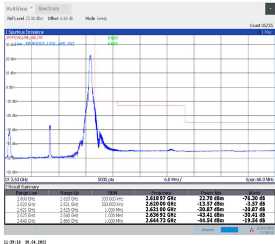
1-N38--30-20-H-2-DFT-PI2BPSK-Edge_1RB_Right-1@50-Ant0-PASS-see graph
