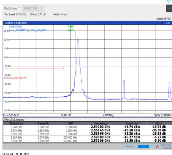
1-N38--30-40-L-4-CP-QPSK-Edge_1RB_Left-1@0-Ant0-PASS-see graph
