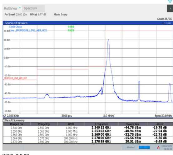
1-N38--30-20-L-4-CP-QPSK-Edge_1RB_Left-1@0-Ant0-PASS-see graph
