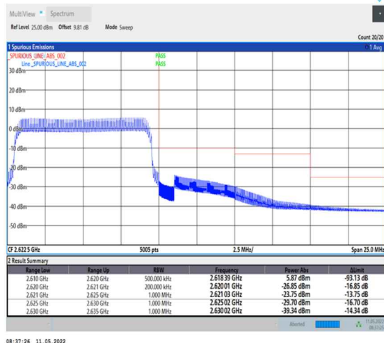
1-N38-PC2-30-10-H-6-CP-QPSK-Outer_Full-24@0-Ant0-PASS-see graph
