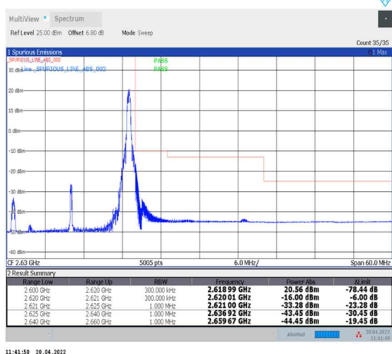
1-N38--30-20-H-5-CP-QPSK-Edge_1RB_Right-1@50-Ant0-PASS-see graph
