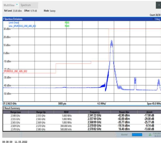
1-N38-PC2-30-15-L-4-CP-QPSK-Edge_1RB_Left-1@0-Ant0-PASS-see graph
