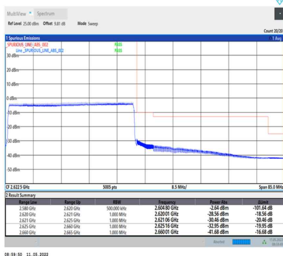
1-N38-PC2-30-40-H-6-CP-QPSK-Outer_Full-106@0-Ant0-PASS-see graph
