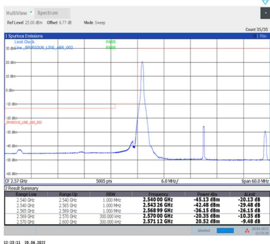
1-N38--30-30-L-4-CP-QPSK-Edge_1RB_Left-1@0-Ant0-PASS-see graph
