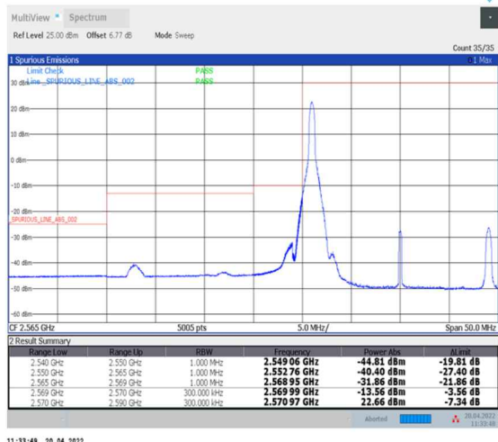
1-N38--30-20-L-1-DFT-PI2BPSK-Edge_1RB_Left-1@0-Ant0-PASS-see graph
