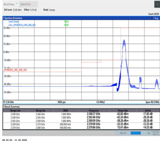
1-N38-PC2-30-10-L-4-CP-QPSK-Edge_1RB_Left-1@0-Ant0-PASS-see graph
