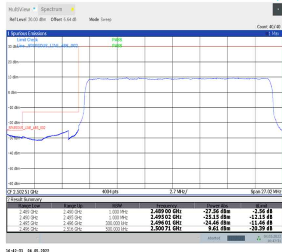
1-N41--30-20-L-3-DFT-PI2BPSK-Outer_Full-50@0-Ant0-PASS-see graph
