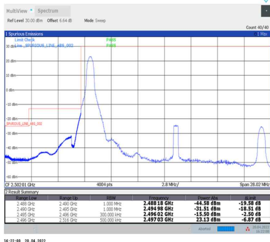
1-N41--30-20-L-4-CP-QPSK-Edge_1RB_Left-1@0-Ant0-PASS-see graph
