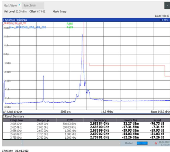
1-N41--30-70-H-2-DFT-PI2BPSK-Edge_1RB_Right-1@188-Ant0-PASS-see graph
