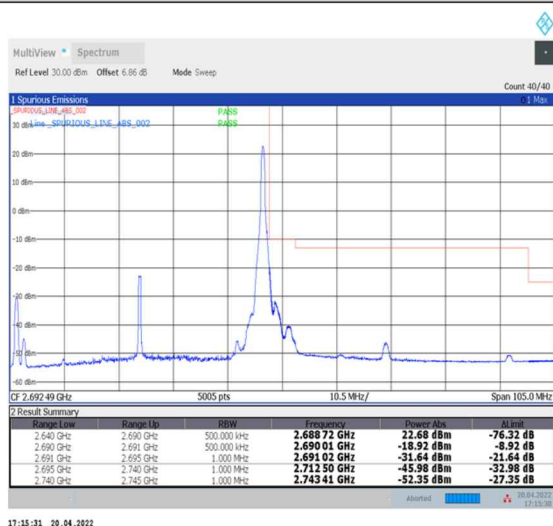
1-N41--30-50-H-5-CP-QPSK-Edge_1RB_Right-1@132-Ant0-PASS-see graph
