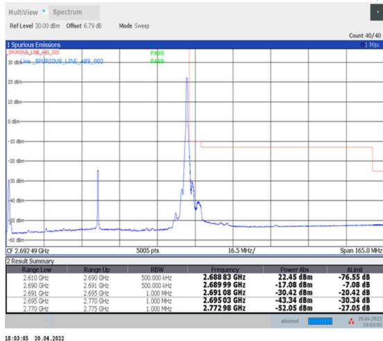
1-N41--30-80-H-2-DFT-PI2BPSK-Edge_1RB_Right-1@216-Ant0-PASS-see graph
