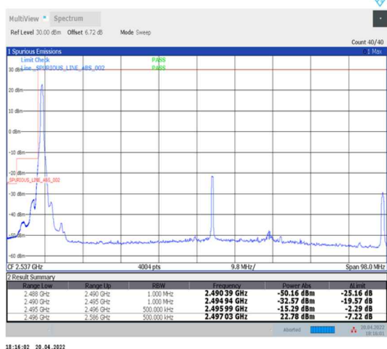
1-N41--30-90-L-4-CP-QPSK-Edge_1RB_Left-1@0-Ant0-PASS-see graph
