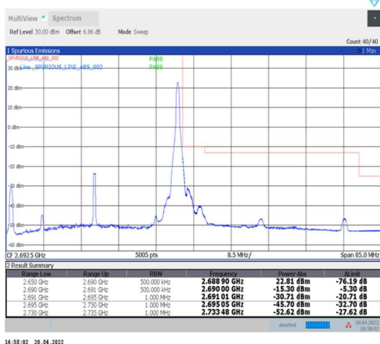
1-N41--30-40-H-5-CP-QPSK-Edge_1RB_Right-1@105-Ant0-PASS-see graph
