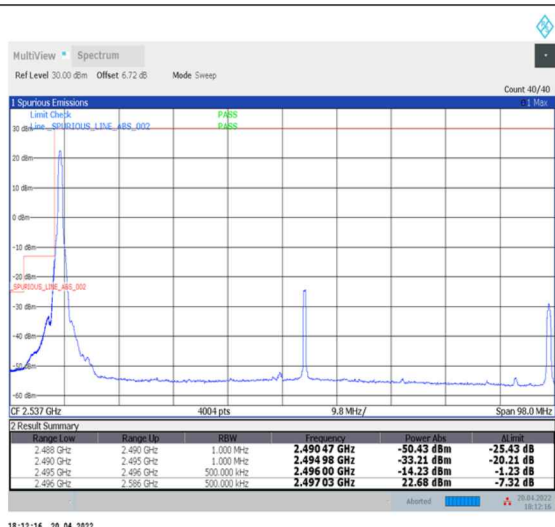
1-N41--30-90-L-1-DFT-PI2BPSK-Edge_1RB_Left-1@0-Ant0-PASS-see graph
