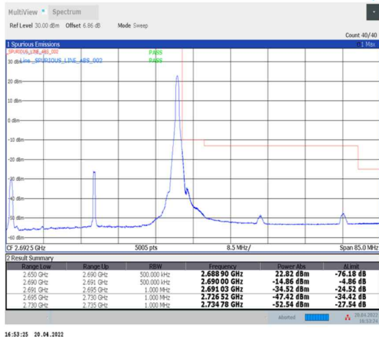
1-N41--30-40-H-2-DFT-PI2BPSK-Edge_1RB_Right-1@105-Ant0-PASS-see graph
