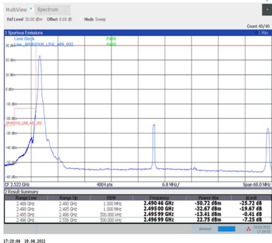
1-N41--30-60-L-1-DFT-PI2BPSK-Edge_1RB_Left-1@0-Ant0-PASS-see graph
