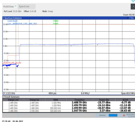
1-N41--30-60-L-6-CP-QPSK-Outer_Full-162@0-Ant0-PASS-see graph
