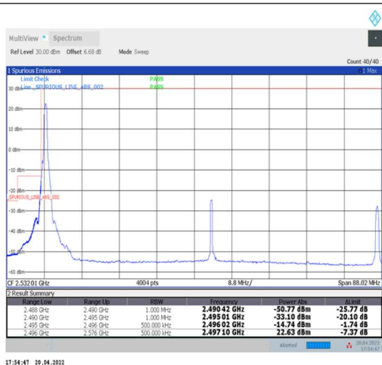
1-N41--30-80-L-1-DFT-PI2BPSK-Edge_1RB_Left-1@0-Ant0-PASS-see graph
