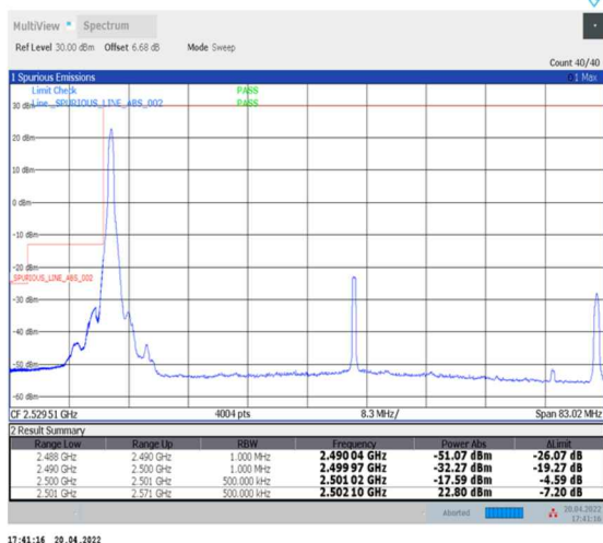
1-N41--30-70-L-4-CP-QPSK-Edge_1RB_Left-1@0-Ant0-PASS-see graph
