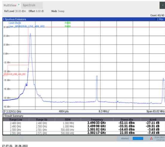
1-N41--30-70-L-1-DFT-PI2BPSK-Edge_1RB_Left-1@0-Ant0-PASS-see graph
