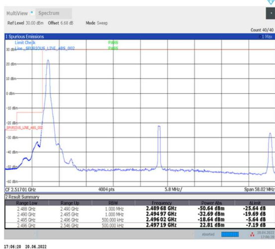
1-N41--30-50-L-4-CP-QPSK-Edge_1RB_Left-1@0-Ant0-PASS-see graph
