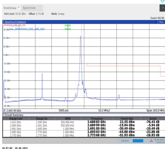
1-N41--30-80-H-5-CP-QPSK-Edge_1RB_Right-1@216-Ant0-PASS-see graph
