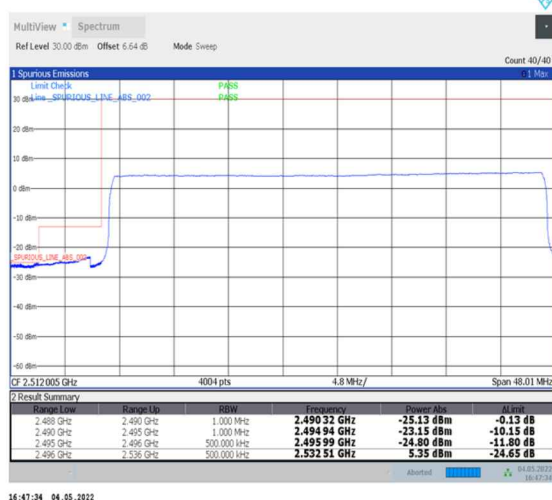
1-N41--30-40-L-6-CP-QPSK-Outer_Full-106@0-Ant0-PASS-see graph
