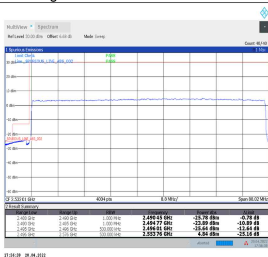
1-N41--30-80-L-3-DFT-PI2BPSK-Outer_Full-216@0-Ant0-PASS-see graph
