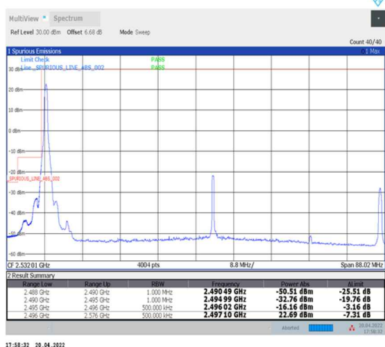
1-N41--30-80-L-4-CP-QPSK-Edge_1RB_Left-1@0-Ant0-PASS-see graph
