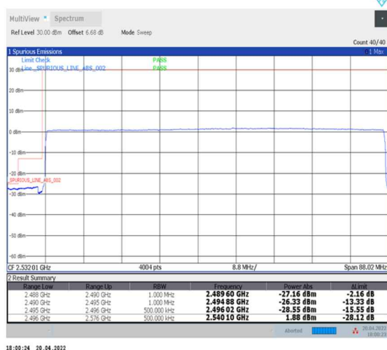
1-N41--30-80-L-6-CP-QPSK-Outer_Full-217@0-Ant0-PASS-see graph
