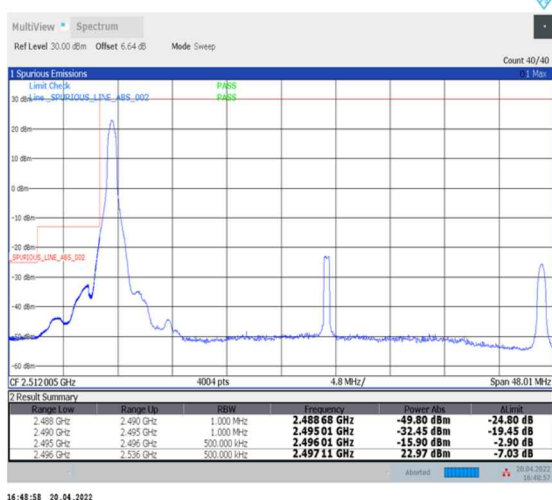
1-N41--30-40-L-4-CP-QPSK-Edge_1RB_Left-1@0-Ant0-PASS-see graph
