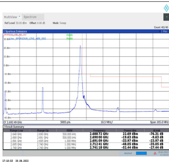
1-N41--30-50-H-2-DFT-PI2BPSK-Edge_1RB_Right-1@132-Ant0-PASS-see graph
