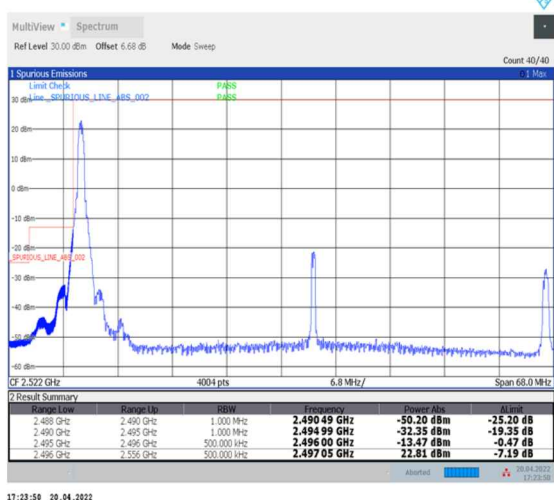
1-N41--30-60-L-4-CP-QPSK-Edge_1RB_Left-1@0-Ant0-PASS-see graph
