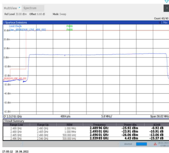
1-N41--30-50-L-6-CP-QPSK-Outer_Full-133@0-Ant0-PASS-see graph
