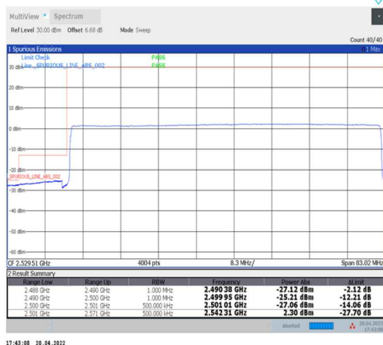
1-N41--30-70-L-6-CP-QPSK-Outer_Full-189@0-Ant0-PASS-see graph
