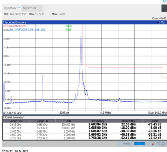
1-N41--30-70-H-5-CP-QPSK-Edge_1RB_Right-1@188-Ant0-PASS-see graph
