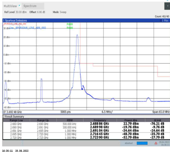
1-N41--30-30-H-2-DFT-PI2BPSK-Edge_1RB_Right-1@77-Ant0-PASS-see graph
