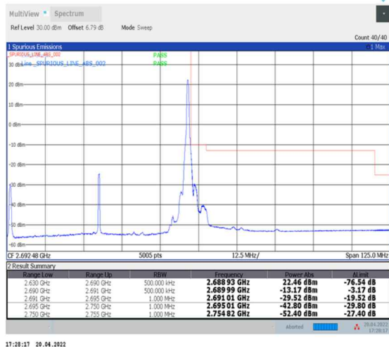
1-N41--30-60-H-2-DFT-PI2BPSK-Edge_1RB_Right-1@161-Ant0-PASS-see graph
