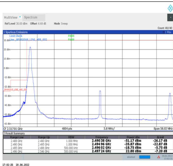
1-N41--30-50-L-1-DFT-PI2BPSK-Edge_1RB_Left-1@0-Ant0-PASS-see graph
