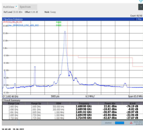
1-N41--30-30-H-5-CP-QPSK-Edge_1RB_Right-1@77-Ant0-PASS-see graph
