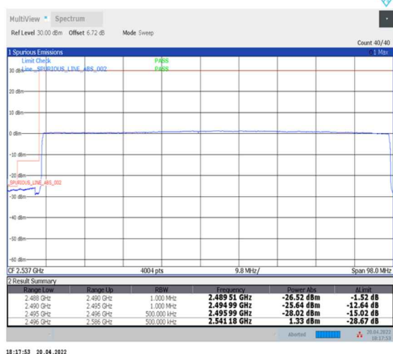
1-N41--30-90-L-6-CP-QPSK-Outer_Full-245@0-Ant0-PASS-see graph
