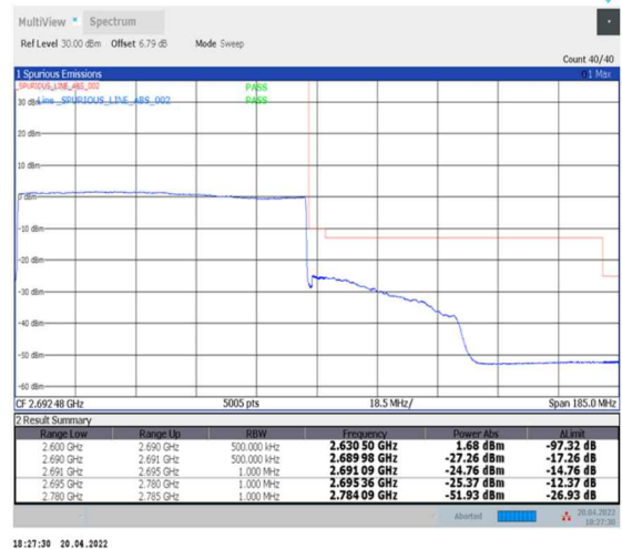
1-N41--30-90-H-6-CP-QPSK-Outer_Full-245@0-Ant0-PASS-see graph
