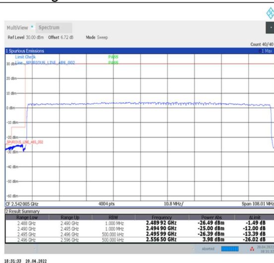
1-N41--30-100-L-3-DFT-PI2BPSK-Outer_Full-270@0-Ant0-PASS-see graph
