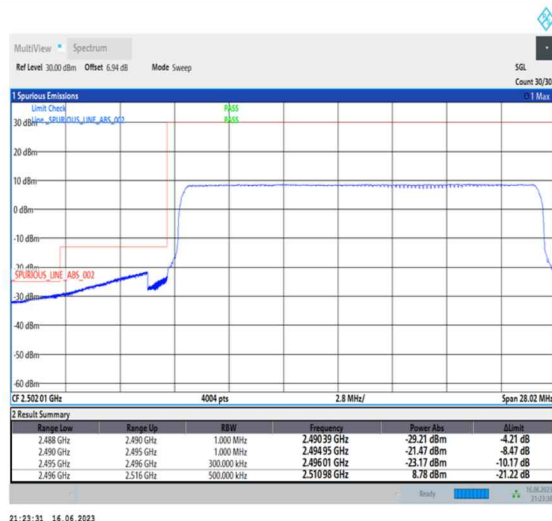
1-N41-PC1-30-20-L-6-CP-QPSK-Outer_Full-51@0-Ant0-1--PASS-see graph
