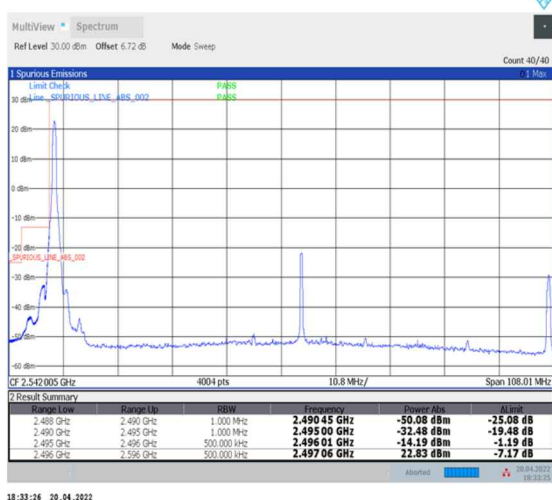
1-N41--30-100-L-4-CP-QPSK-Edge_1RB_Left-1@0-Ant0-PASS-see graph
