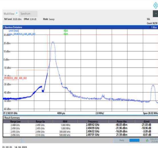
1-N41-PC1-30-20-L-4-CP-QPSK-Edge_1RB_Left-1@0-Ant0-1--PASS-see graph
