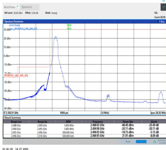
1-N41-PC1-30-20-L-1-DFT-PI2BPSK-Edge_1RB_Left-1@0-Ant0-1--PASS-see graph
