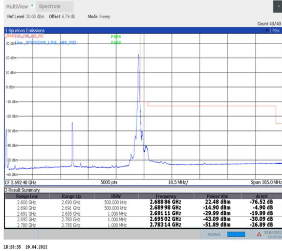
1-N41--30-90-H-2-DFT-PI2BPSK-Edge_1RB_Right-1@244-Ant0-PASS-see graph
