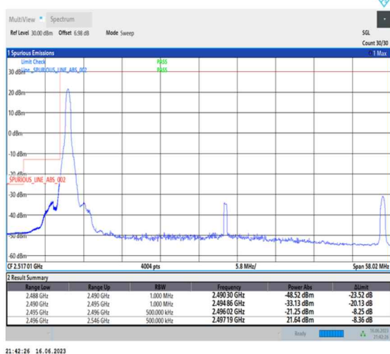
1-N41-PC1-30-50-L-4-CP-QPSK-Edge_1RB_Left-1@0-Ant0-1--PASS-see graph
