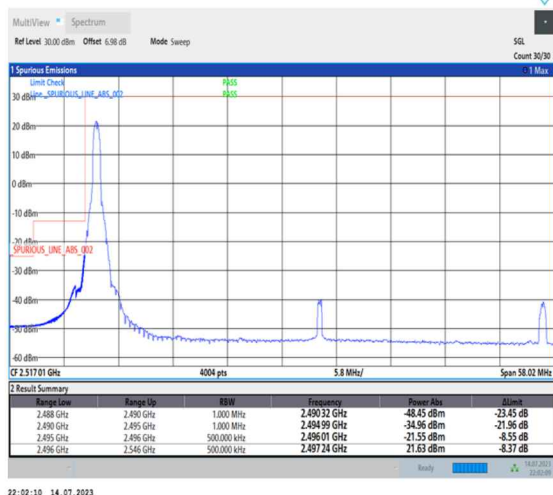
1-N41-PC1-30-50-L-1-DFT-PI2BPSK-Edge_1RB_Left-1@0-Ant0-1--PASS-see graph
