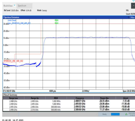
1-N41-PC1-30-20-L-3-DFT-PI2BPSK-Outer_Full-50@0-Ant0-1--PASS-see graph
