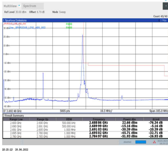
1-N41--30-90-H-5-CP-QPSK-Edge_1RB_Right-1@244-Ant0-PASS-see graph
