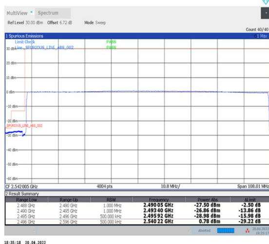
1-N41--30-100-L-6-CP-QPSK-Outer_Full-273@0-Ant0-PASS-see graph
