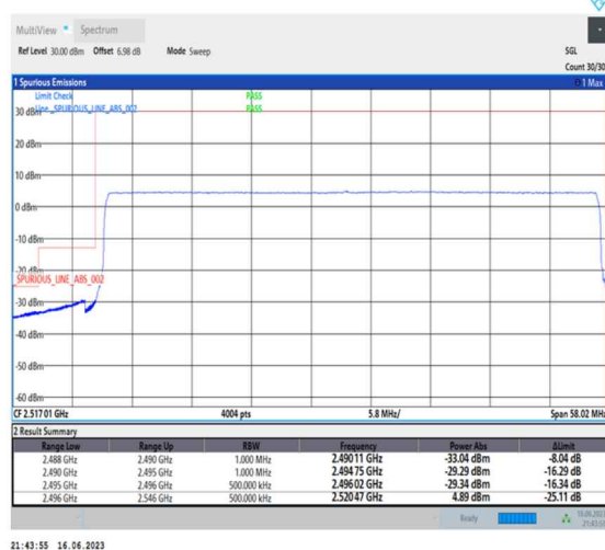
1-N41-PC1-30-50-L-6-CP-QPSK-Outer_Full-133@0-Ant0-1--PASS-see graph
