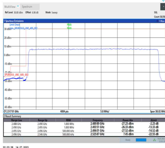
1-N41-PC1-30-50-L-3-DFT-PI2BPSK-Outer_Full-128@0-Ant0-1--PASS-see graph
