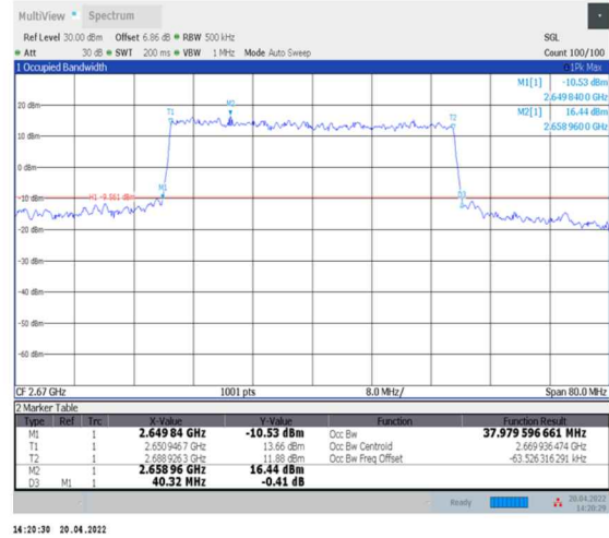
1-N41--30-40-H-6-CP-QPSK-Outer_Full-106@0-Ant0-37.98-40.320-≤40-PASS
