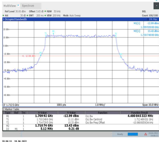
1-N66-PC3-15-5-L-1-DFT-QPSK-Outer_Full-25@0- Ant0-4.481-5.120-≤5-PASS
