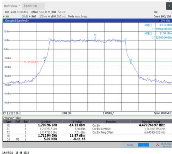
1-N66-PC3-15-5-L-3-DFT-16QAM-Outer_Full-25@0- Ant0-4.48-5.090-≤5-PASS
