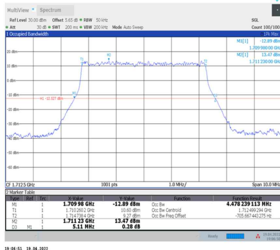
1-N66-PC3-15-5-L-2-DFT-PI2BPSK-Outer_Full- 25@0-Ant0-4.478-5.110-≤5-PASS
