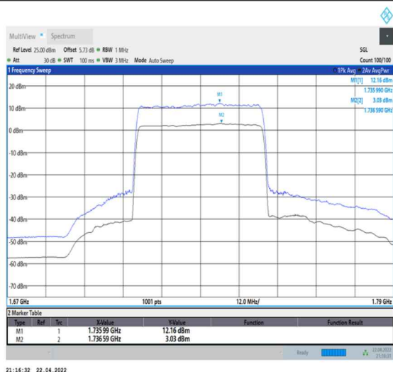
1-N66-PC3-15-40-L-1-DFT-256QAM-Outer_Full-216@0-Ant0-9.13-100%-0.00-9.13-PASS-≤13
