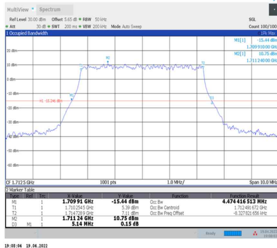
1-N66-PC3-15-5-L-4-DFT-64QAM-Outer_Full-25@0- Ant0-4.474-5.140-≤5-PASS
