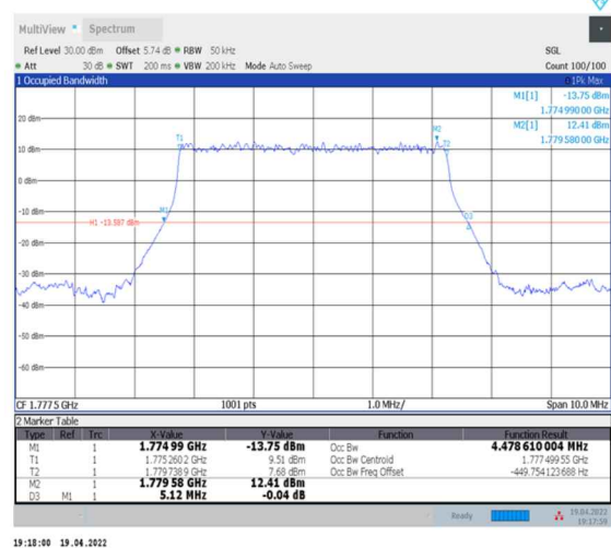
1-N66-PC3-15-5-H-2-DFT-PI2BPSK-Outer_Full-25@0-Ant0-4.479-5.120-≤5-PASS
