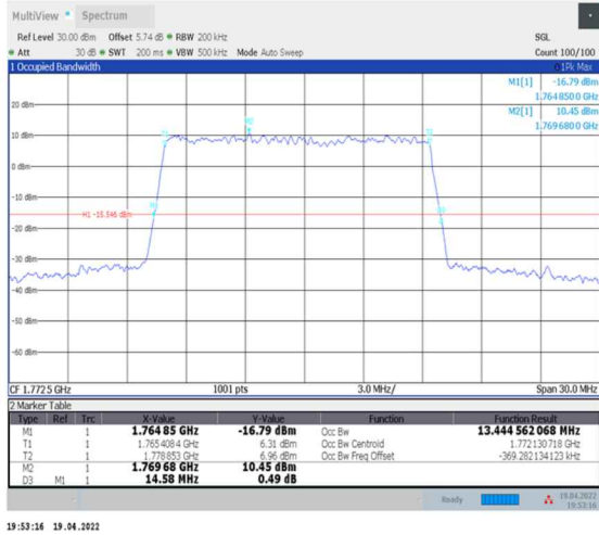
1-N66-PC3-15-15-H-5-DFT-256QAM-Outer_Full-75@0-Ant0-13.445-14.580-≤15-PASS
