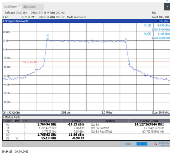
1-N66-PC3-15-15-H-7-CP-16QAM-Outer_Full-79@0-Ant0-14.127-15.180-≤15-PASS
