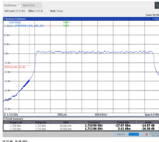
1-N66-PC3-15-5-L-3-DFT-PI2BPSK-Outer_Full-25@0-Ant0-seegraph-PASS-see graph
