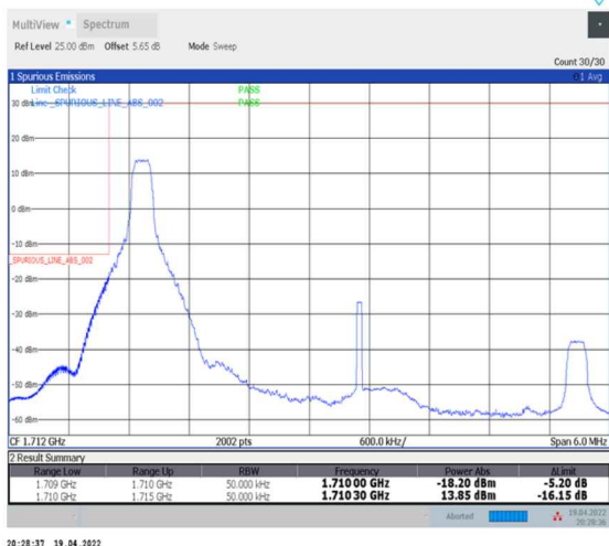
1-N66-PC3-15-5-L-4-CP-QPSK-Edge_1RB_Left-1@0-Ant0-seegraph-PASS-see graph
