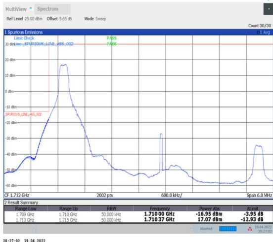
1-N66-PC3-15-5-L-1-DFT-PI2BPSK-Edge_1RB_Left-1@0-Ant0-seegraph-PASS-see graph
