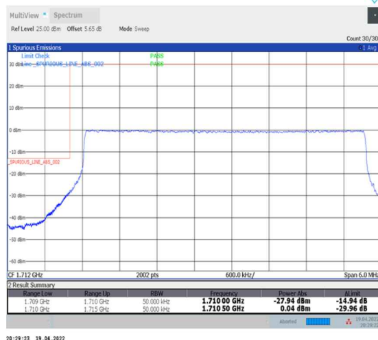
1-N66-PC3-15-5-L-6-CP-QPSK-Outer_Full-25@0-Ant0-seegraph-PASS-see graph
