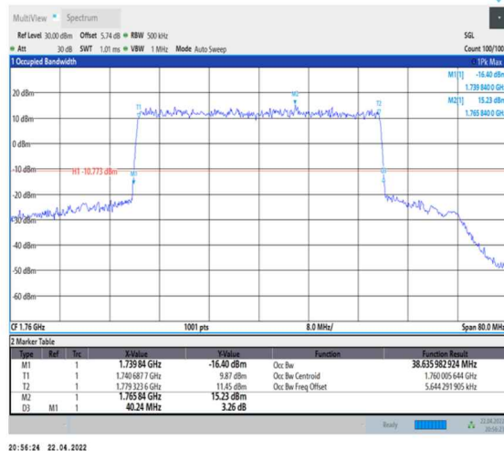
1-N66-PC3-15-40-H-1-DFT-QPSK-Outer_Full-216@0-Ant0-38.636-40.240-≤40-PASS
