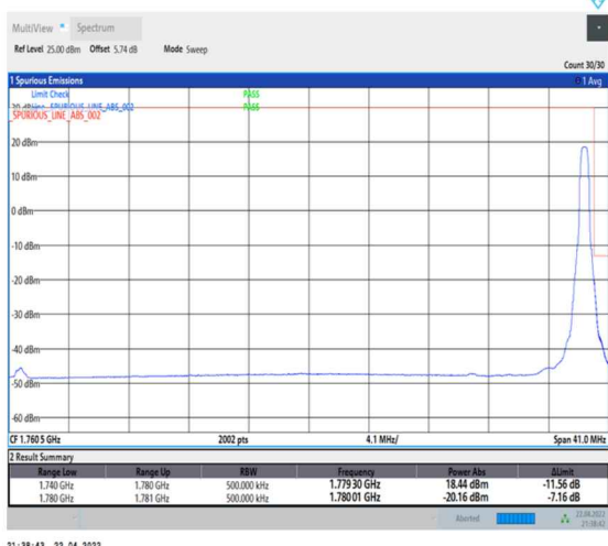
1-N66-PC3-15-40-H-5-CP-QPSK-Edge_1RB_Right-1@215-Ant0-seegraph-PASS-see graph
