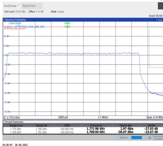
1-N66-PC3-15-10-H-3-DFT-PI2BPSK-Outer_Full-50@0-Ant0-seegraph-PASS-see graph
