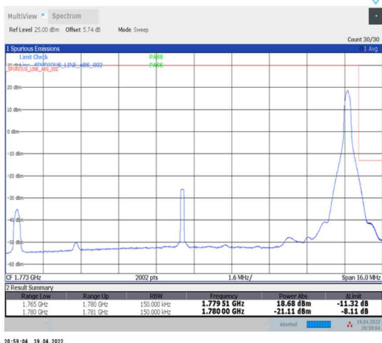
1-N66-PC3-15-15-H-5-CP-QPSK-Edge_1RB_Right-1@78-Ant0-seegraph-PASS-see graph
