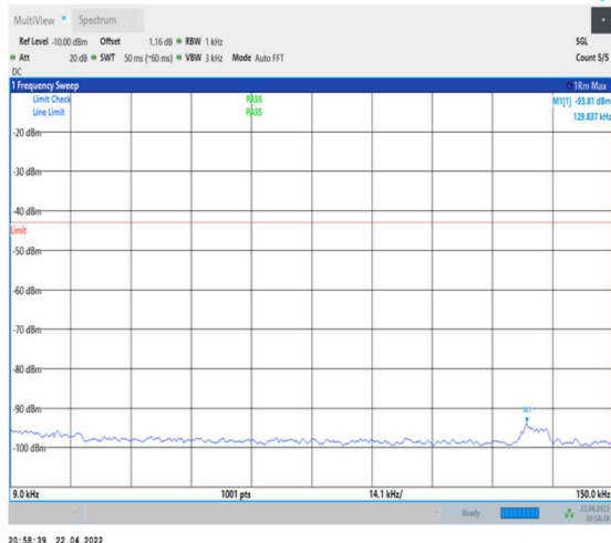
1-N66-PC3-15-40-L-1-DFT-PI2BPSK- Inner_1RB_Left-1@1-0.009-0.15-Ant0--93.81--43- PASS
