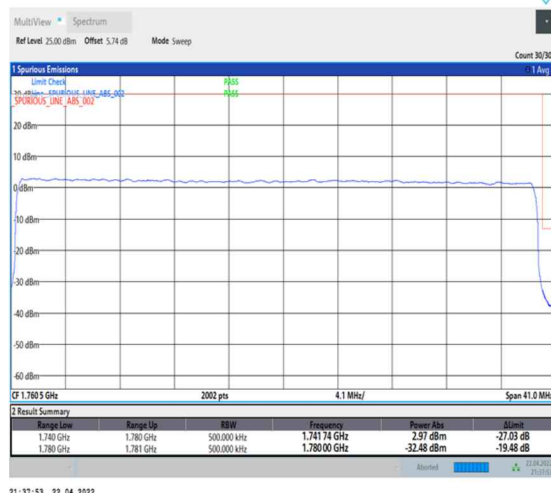
1-N66-PC3-15-40-H-3-DFT-PI2BPSK-Outer_Full-216@0-Ant0-seegraph-PASS-see graph
