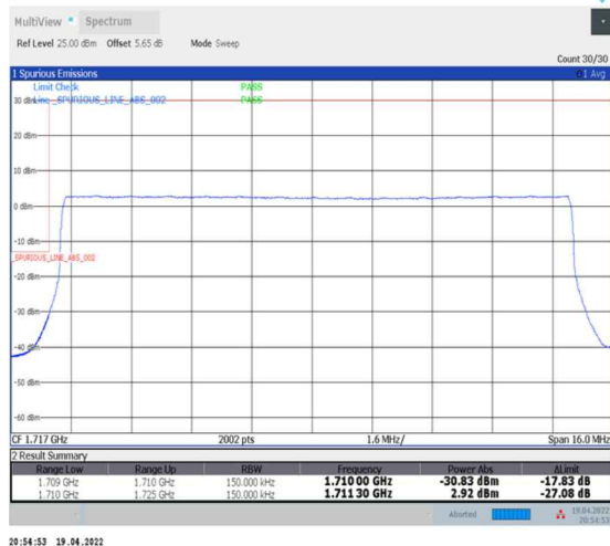
1-N66-PC3-15-15-L-3-DFT-PI2BPSK-Outer_Full-75@0-Ant0-seegraph-PASS-see graph
