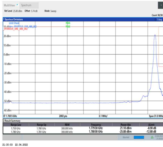
1-N66-PC3-15-30-H-2-DFT-PI2BPSK-Edge_1RB_Right-1@159-Ant0-seegraph-PASS-see graph
