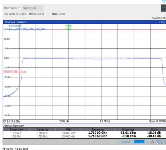
1-N66-PC3-15-10-L-6-CP-QPSK-Outer_Full-52@0-Ant0-seegraph-PASS-see graph
