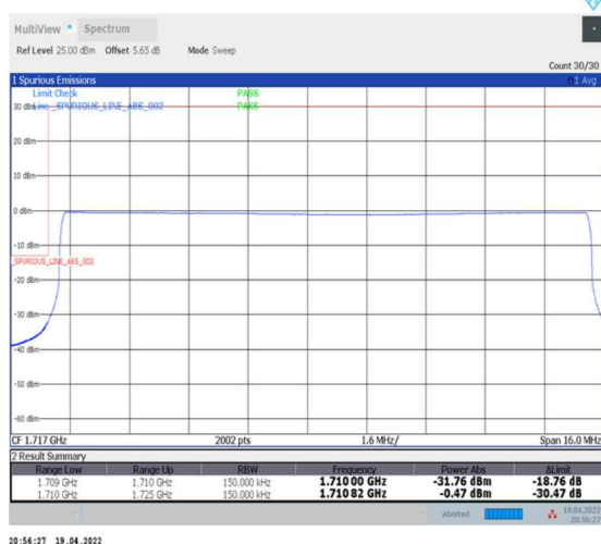
1-N66-PC3-15-15-L-6-CP-QPSK-Outer_Full-79@0-Ant0-seegraph-PASS-see graph
