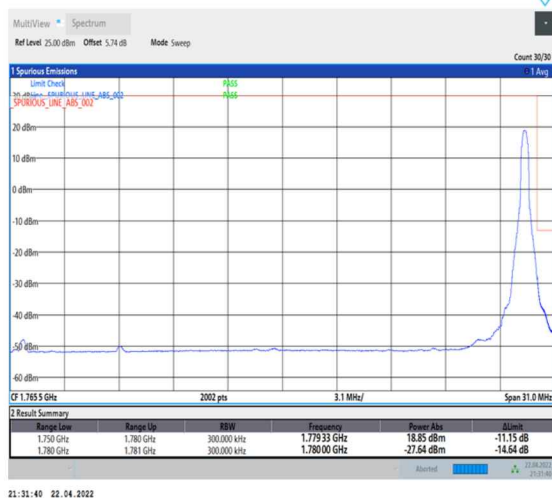
1-N66-PC3-15-30-H-5-CP-QPSK-Edge_1RB_Right-1@159-Ant0-seegraph-PASS-see graph
