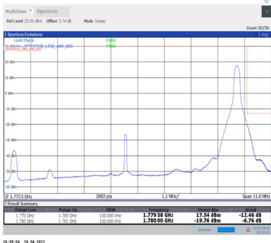
1-N66-PC3-15-10-H-5-CP-QPSK-Edge_1RB_Right-1@51-Ant0-seegraph-PASS-see graph
