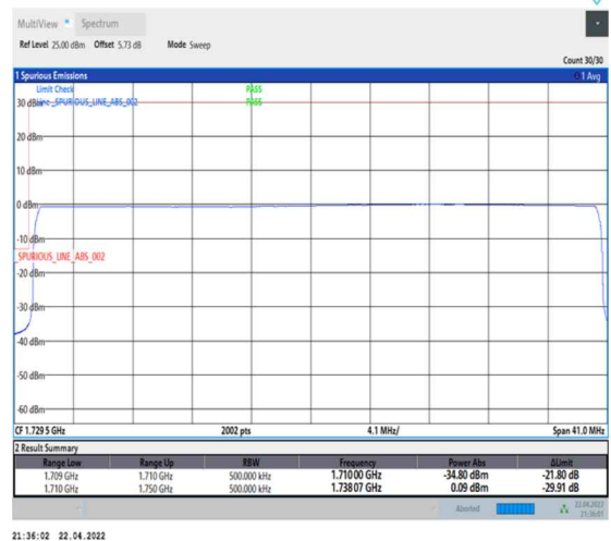
1-N66-PC3-15-40-L-6-CP-QPSK-Outer_Full-216@0-Ant0-seegraph-PASS-see graph
