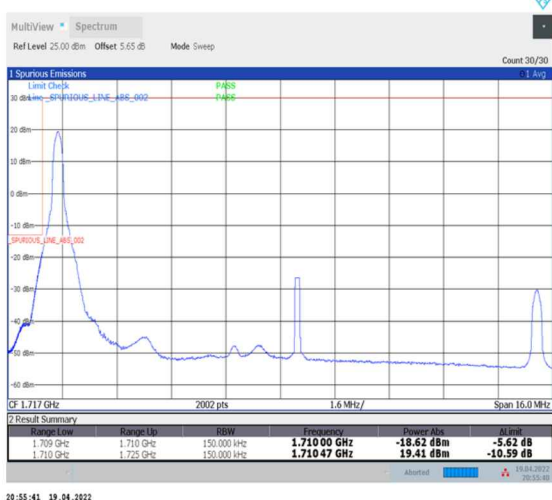
1-N66-PC3-15-15-L-4-CP-QPSK-Edge_1RB_Left-1@0-Ant0-seegraph-PASS-see graph
