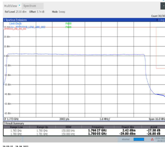
1-N66-PC3-15-15-H-3-DFT-PI2BPSK-Outer_Full-75@0-Ant0-seegraph-PASS-see graph
