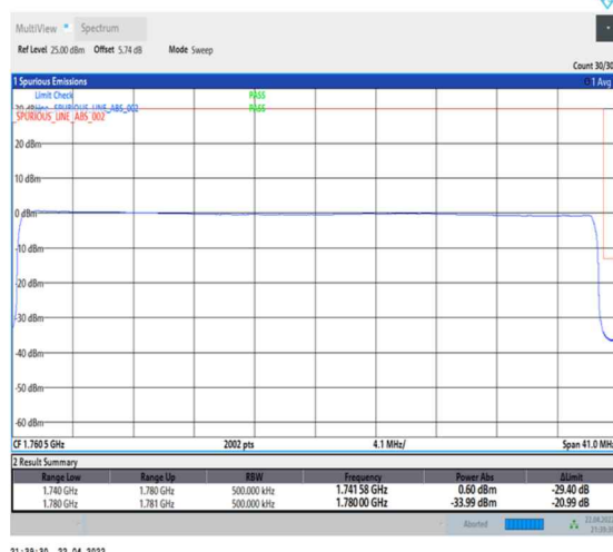
1-N66-PC3-15-40-H-6-CP-QPSK-Outer_Full-216@0-Ant0-seegraph-PASS-see graph
