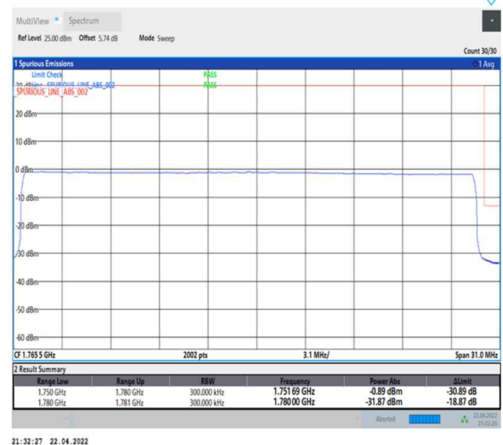
1-N66-PC3-15-30-H-6-CP-QPSK-Outer_Full-160@0-Ant0-seegraph-PASS-see graph
