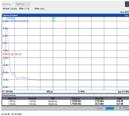
1-N66-PC3-15-40-L-1-DFT-PI2BPSK-Edge_1RB_Left-1@0-Ant0-seegraph-PASS-see graph
