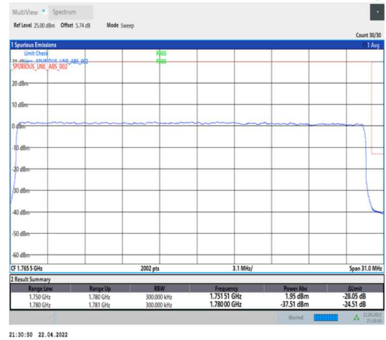
1-N66-PC3-15-30-H-3-DFT-PI2BPSK-Outer_Full-160@0-Ant0-seegraph-PASS-see graph
