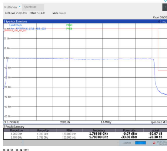
1-N66-PC3-15-15-H-6-CP-QPSK-Outer_Full-79@0-Ant0-seegraph-PASS-see graph
