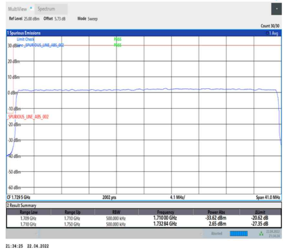
1-N66-PC3-15-40-L-3-DFT-PI2BPSK-Outer_Full-216@0-Ant0-seegraph-PASS-see graph
