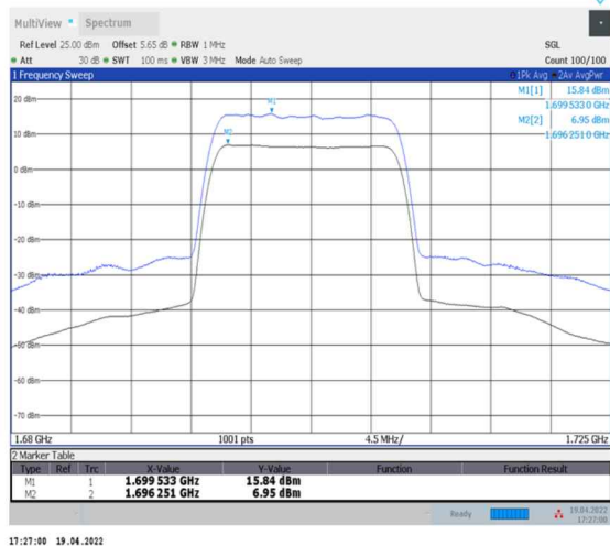
1-N70--15-15-M-1-DFT-256QAM-Outer_Full-75@0- Ant2-8.89-100%-0.00-8.89-PASS-≤13
