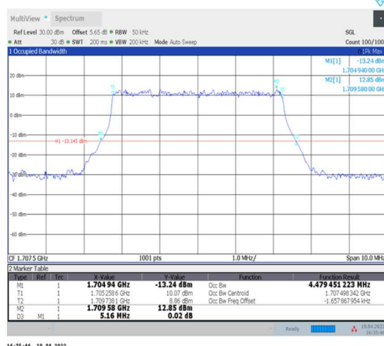
1-N70--15-5-H-2-DFT-PI2BPSK-Outer_Full-25@0-Ant2-4.479-5.160-≤5-PASS
