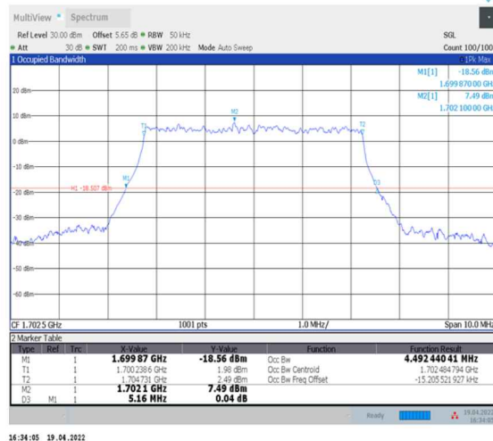
1-N70--15-5-M-9-CP-256QAM-Outer_Full-25@0-Ant2-4.492-5.160-≤5-PASS
