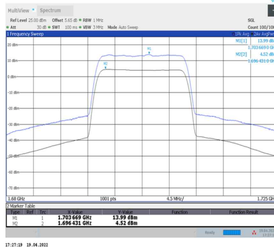
1-N70--15-15-M-2-CP-256QAM-Outer_Full-79@0- Ant2-9.47-100%-0.00-9.47-PASS-≤13
