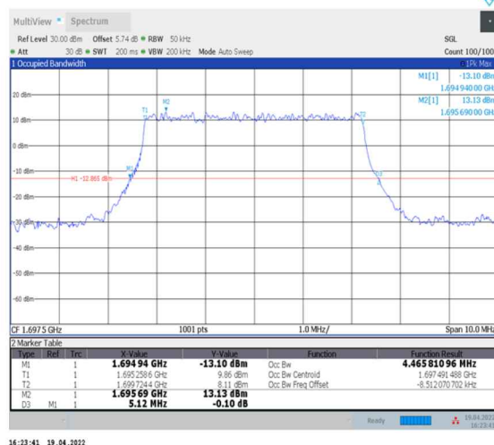
1-N70--15-5-L-2-DFT-PI2BPSK-Outer_Full-25@0-Ant2-4.466-5.120-≤5-PASS
