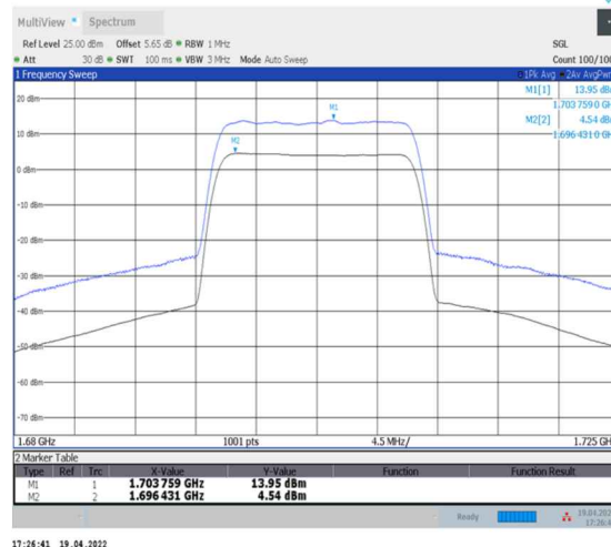
1-N70--15-15-L-2-CP-256QAM-Outer_Full-79@0- Ant2-9.41-100%-0.00-9.41-PASS-≤13
