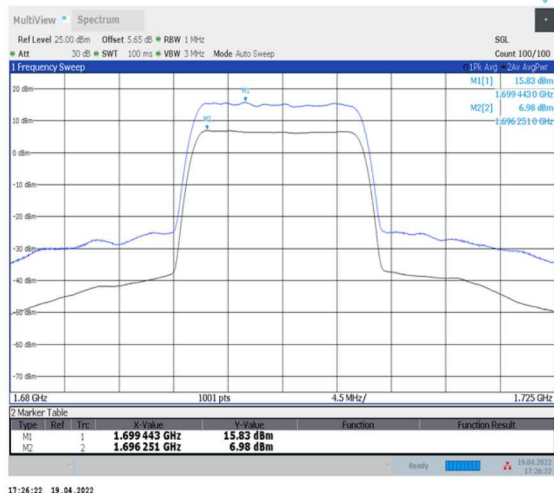
1-N70--15-15-L-1-DFT-256QAM-Outer_Full-75@0- Ant2-8.85-100%-0.00-8.85-PASS-≤13
