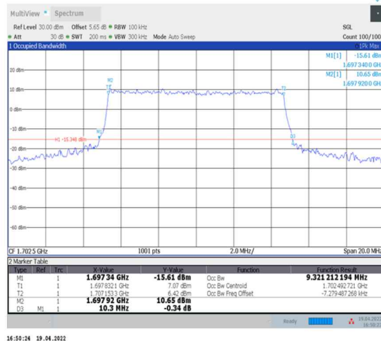
1-N70--15-10-M-6-CP-QPSK-Outer_Full-52@0-Ant2-9.321-10.300-≤10-PASS
