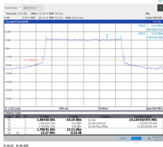
1-N70--15-15-L-6-CP-QPSK-Outer_Full-79@0-Ant2-14.134-15.270-≤15-PASS
