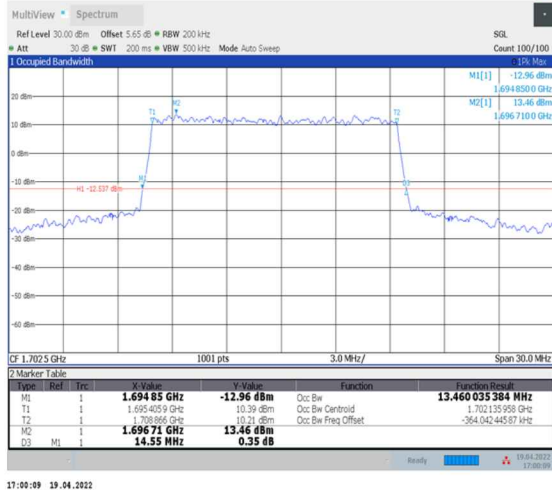
1-N70--15-15-L-3-DFT-16QAM-Outer_Full-75@0-Ant2-13.46-14.550-≤15-PASS
