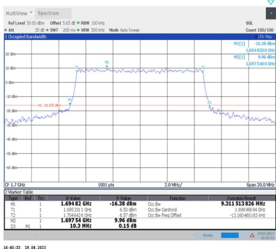
1-N70--15-10-L-8-CP-64QAM-Outer_Full-52@0-Ant2-9.312-10.300-≤10-PASS
