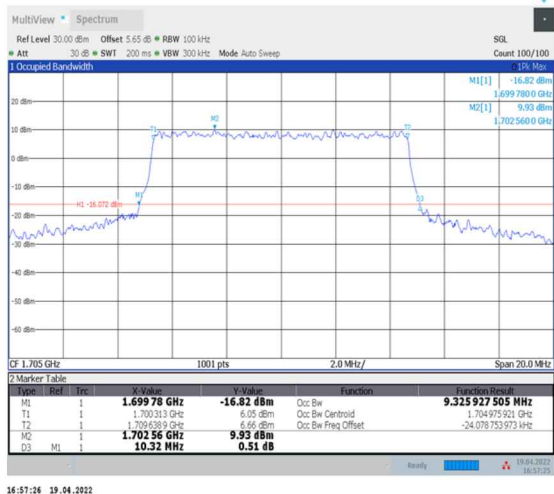
1-N70--15-10-H-8-CP-64QAM-Outer_Full-52@0-Ant2-9.326-10.320-≤10-PASS
