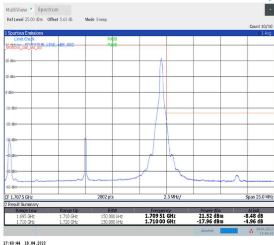
1-N70--15-15-H-2-DFT-PI2BPSK-Edge_1RB_Right-1@78-Ant2-seegraph-PASS-see graph
