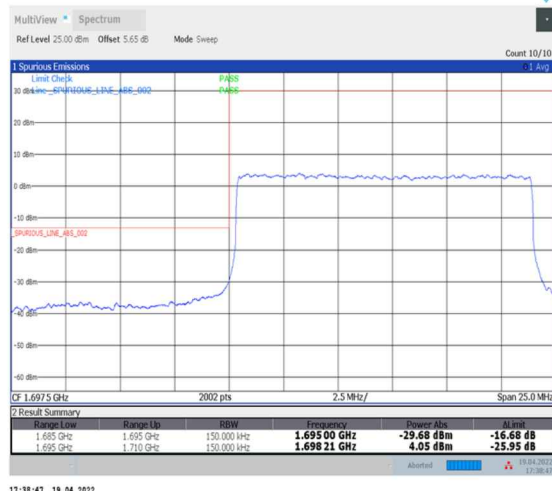
1-N70--15-15-L-3-DFT-PI2BPSK-Outer_Full-75@0-Ant2-seegraph-PASS-see graph
