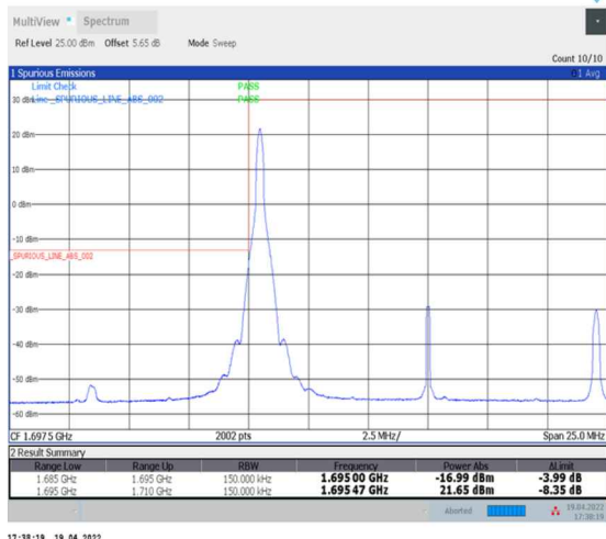
1-N70--15-15-L-1-DFT-PI2BPSK-Edge_1RB_Left-1@0-Ant2-seegraph-PASS-see graph
