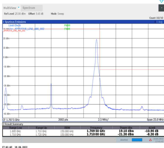
1-N70--15-15-H-5-CP-QPSK-Edge_1RB_Right-1@78-Ant2-seegraph-PASS-see graph
