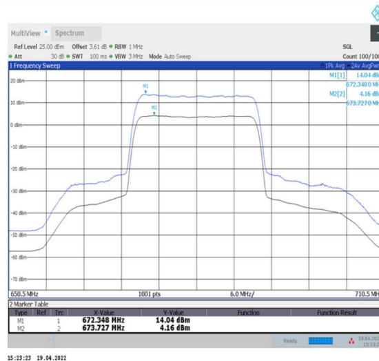
1-N71--15-20-M-2-CP-256QAM-Outer_Full-106@0-Ant0-9.88-100%-0.00-9.88-PASS-≤13
