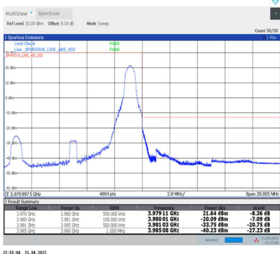
1-N77-3700-3980--30-10-H-5-CP-QPSK-Edge_1RB_Right-1@23-Ant0-PASS-see graph
