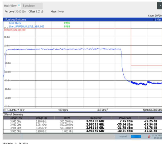
1-N77-3700-3980--30-40-H-3-DFT-PI2BPSK-Outer_Full-100@0-Ant0-PASS-see graph
