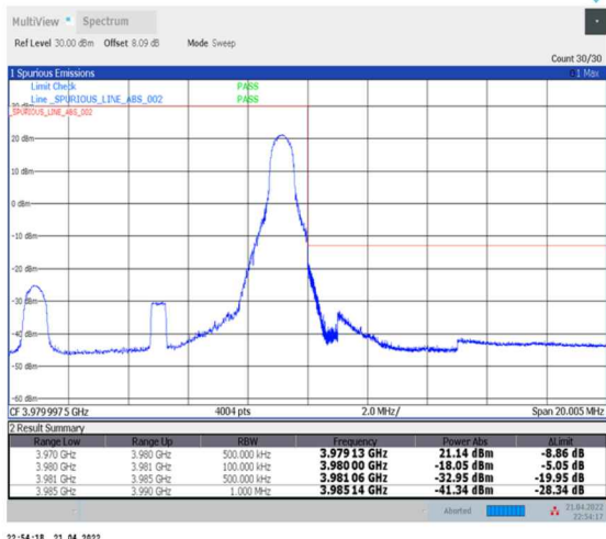
1-N77-3700-3980--30-10-H-2-DFT-PI2BPSK-Edge_1RB_Right-1@23-Ant0-PASS-see graph
