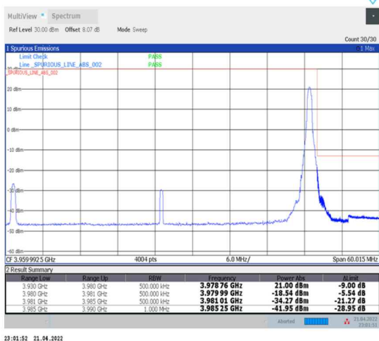
1-N77-3700-3980--30-50-H-2-DFT-PI2BPSK-Edge_1RB_Right-1@132-Ant0-PASS-see graph
