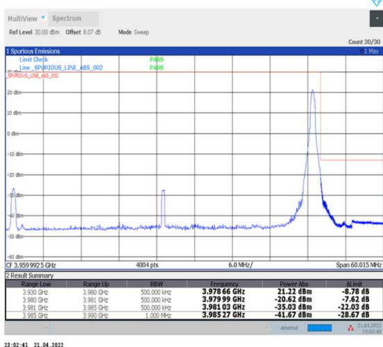
1-N77-3700-3980--30-50-H-5-CP-QPSK-Edge_1RB_Right-1@132-Ant0-PASS-see graph
