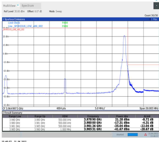
1-N77-3700-3980--30-40-H-2-DFT-PI2BPSK-Edge_1RB_Right-1@105-Ant0-PASS-see graph
