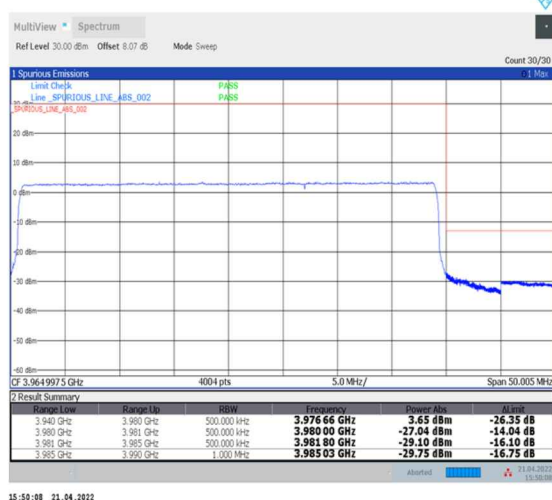
1-N77-3700-3980--30-40-H-6-CP-QPSK-Outer_Full-106@0-Ant0-PASS-see graph
