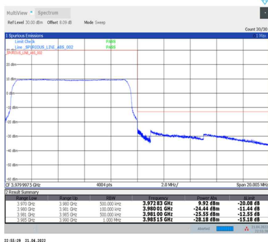
1-N77-3700-3980--30-10-H-6-CP-QPSK-Outer_Full-24@0-Ant0-PASS-see graph
