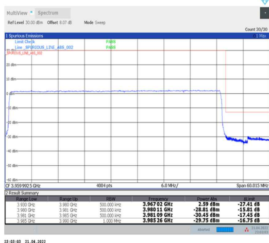
1-N77-3700-3980--30-50-H-6-CP-QPSK-Outer_Full-133@0-Ant0-PASS-see graph
