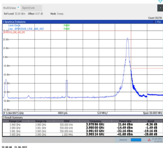
1-N77-3700-3980--30-40-H-5-CP-QPSK-Edge_1RB_Right-1@105-Ant0-PASS-see graph
