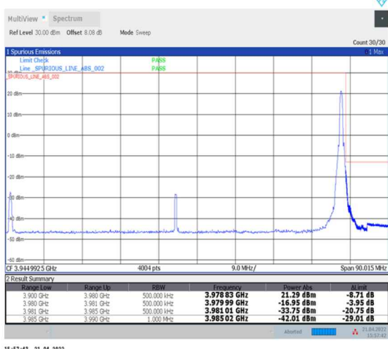
1-N77-3700-3980--30-80-H-5-CP-QPSK-Edge_1RB_Right-1@216-Ant0-PASS-see graph
