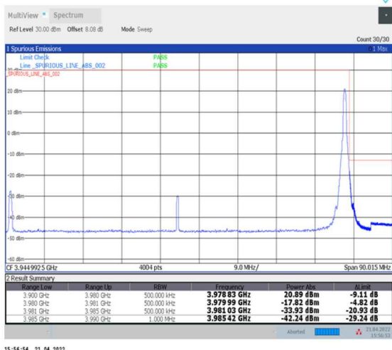
1-N77-3700-3980--30-80-H-2-DFT-PI2BPSK-Edge_1RB_Right-1@216-Ant0-PASS-see graph
