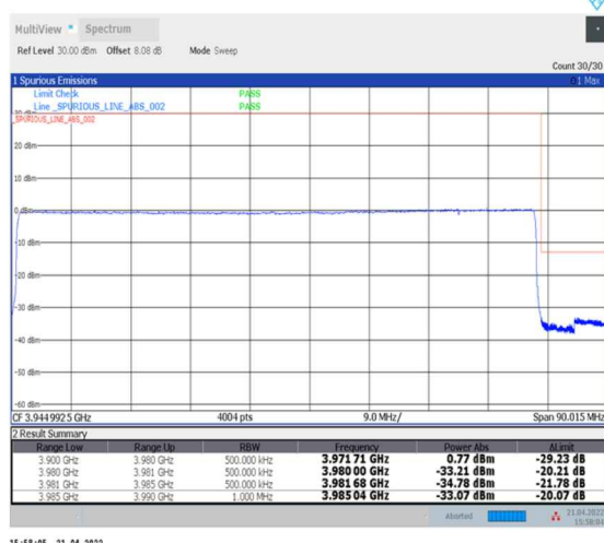
1-N77-3700-3980--30-80-H-6-CP-QPSK-Outer_Full-217@0-Ant0-PASS-see graph
