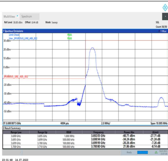
1-N77-3700-3980-PC1-30-10-L-1-DFT-PI2BPSK-Edge_1RB_Left-1@0-Ant0-1--PASS-see graph
