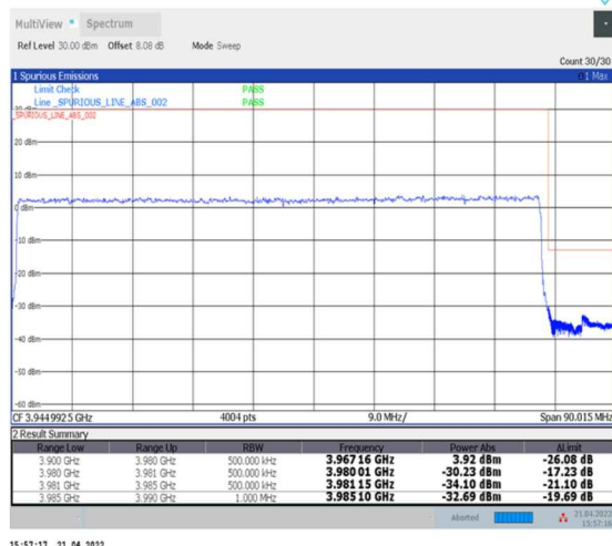
1-N77-3700-3980--30-80-H-3-DFT-PI2BPSK-Outer_Full-216@0-Ant0-PASS-see graph
