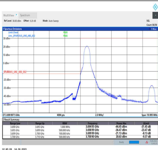
1-N77-3700-3980-PC1-30-10-L-4-CP-QPSK-Edge_1RB_Left-1@0-Ant0-1--PASS-see graph
