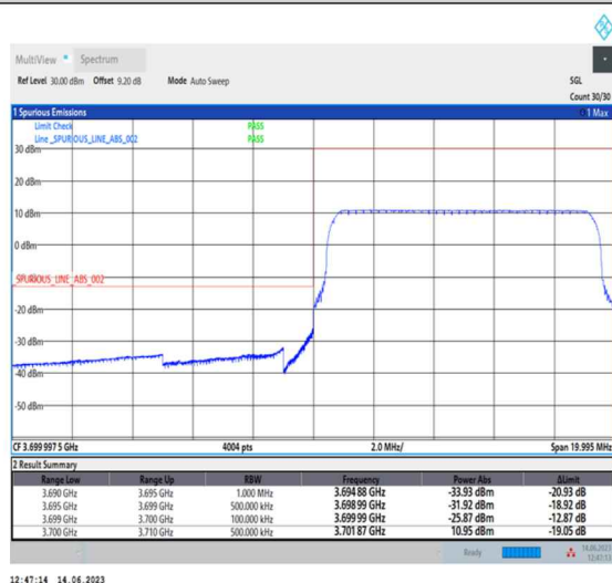
1-N77-3700-3980-PC1-30-10-L-6-CP-QPSK-Outer_Full-24@0-Ant0-1--PASS-see graph
