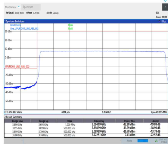
1-N77-3700-3980-PC1-30-40-L-6-CP-QPSK-Outer_Full-106@0-Ant0-1--PASS-see graph
