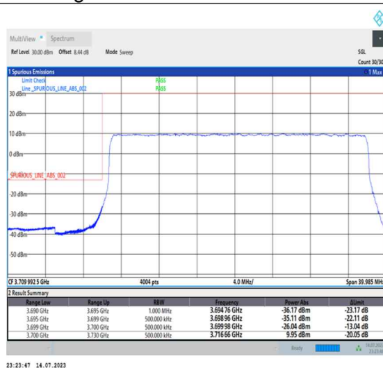
1-N77-3700-3980-PC1-30-30-L-3-DFT-PI2BPSK-Outer_Full-75@0-Ant0-1--PASS-see graph
