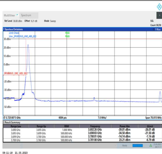
1-N77-3700-3980-PC1-30-60-L-4-CP-QPSK-Edge_1RB_Left-1@0-Ant0-1--PASS-see graph
