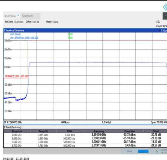
1-N77-3700-3980-PC1-30-60-L-6-CP-QPSK-Outer_Full-162@0-Ant0-1--PASS-see graph
