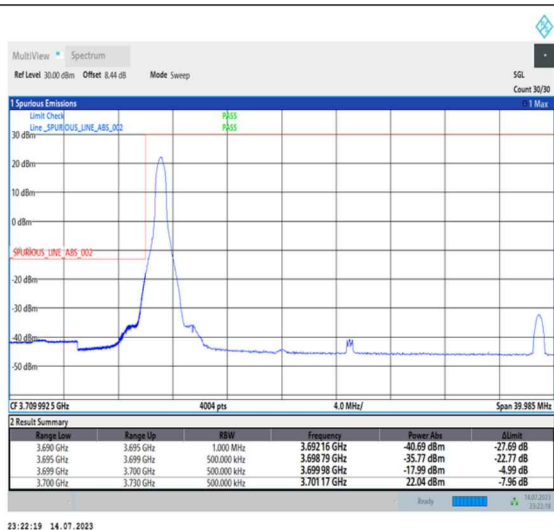
1-N77-3700-3980-PC1-30-30-L-1-DFT-PI2BPSK-Edge_1RB_Left-1@0-Ant0-1--PASS-see graph
