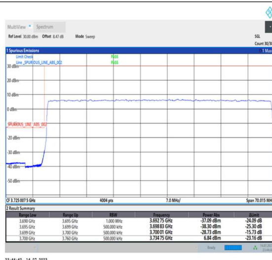
1-N77-3700-3980-PC1-30-60-L-3-DFT-PI2BPSK-Outer_Full-162@0-Ant0-1--PASS-see graph
