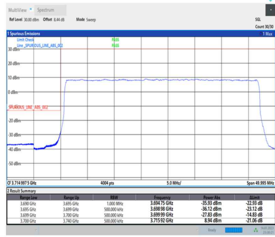
1-N77-3700-3980-PC1-30-40-L-3-DFT-PI2BPSK-Outer_Full-100@0-Ant0-1--PASS-see graph
