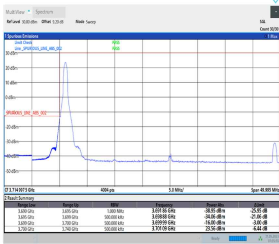
1-N77-3700-3980-PC1-30-40-L-4-CP-QPSK-Edge_1RB_Left-1@0-Ant0-1--PASS-see graph
