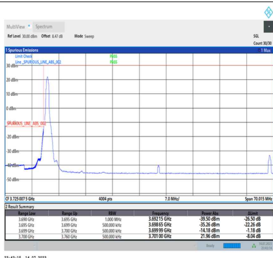
1-N77-3700-3980-PC1-30-60-L-1-DFT-PI2BPSK-Edge_1RB_Left-1@0-Ant0-1--PASS-see graph
