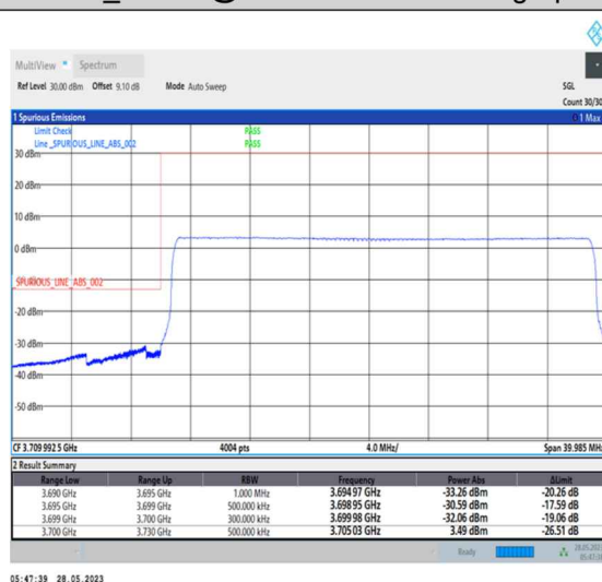
1-N77-3700-3980-PC1-30-30-L-6-CP-QPSK-Outer_Full-78@0-Ant0-1--PASS-see graph
