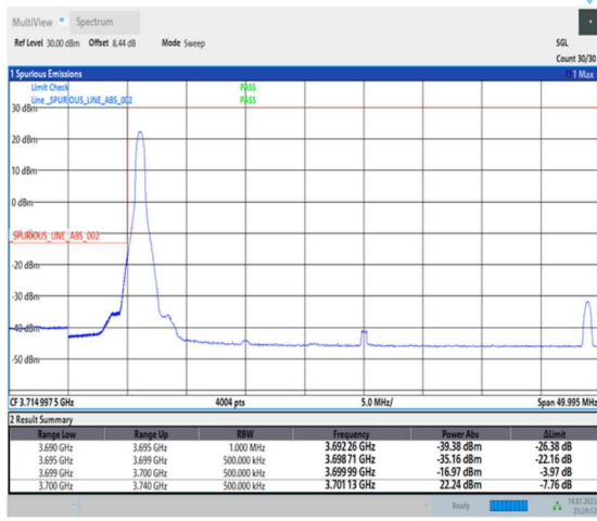
1-N77-3700-3980-PC1-30-40-L-1-DFT-PI2BPSK-Edge_1RB_Left-1@0-Ant0-1--PASS-see graph
