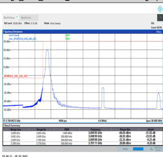
1-N77-3700-3980-PC1-30-30-L-4-CP-QPSK-Edge_1RB_Left-1@0-Ant0-1--PASS-see graph
