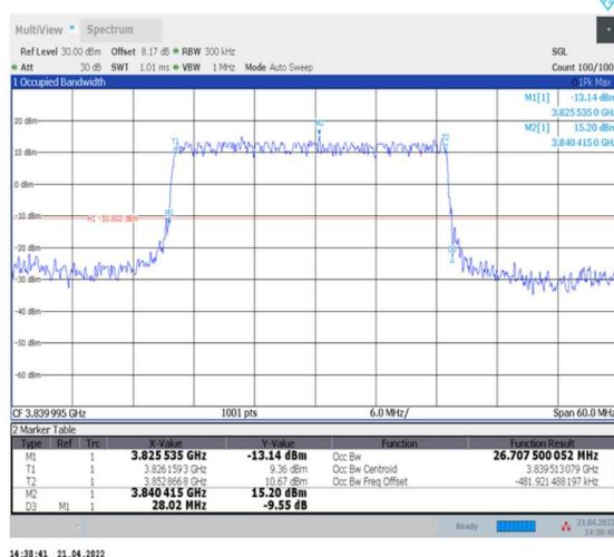
1-N77-3700-3980--30-30-M-2-DFT-PI2BPSK-Outer_Full-75@0-Ant0-26.71-28.020-≤30-PASS
