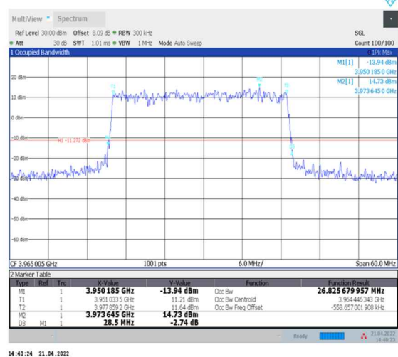
1-N77-3700-3980--30-30-H-1-DFT-QPSK-Outer_Full-75@0-Ant0-26.826-28.500-≤30-PASS
