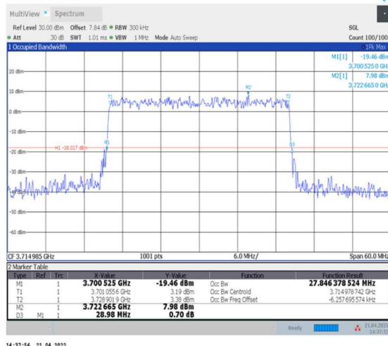
1-N77-3700-3980--30-30-L-9-CP-256QAM-Outer_Full-78@0-Ant0-27.852-28.980-≤30-PASS
