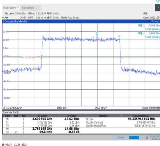
1-N77-3700-3980--30-100-L-1-DFT-QPSK-Outer_Full-270@0-Ant0-96.336-99.800-<100-PASS
