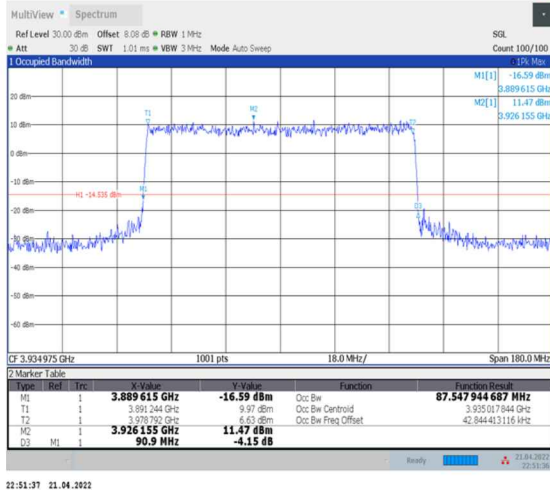
1-N77-3700-3980--30-90-H-8-CP-64QAM-Outer_Full-245@0-Ant0-87.548-90.900-<90-PASS
