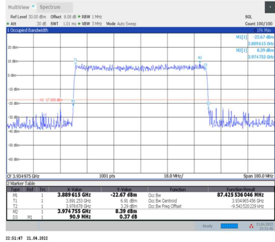
1-N77-3700-3980--30-90-H-9-CP-256QAM-Outer_Full-245@0-Ant0-87.426-90.900-<90-PASS
