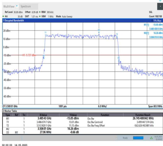
1-N78-3450-3550-PC1-30-30-M-1-DFT-QPSK-Outer_Full-75@0-Ant0-26.745-27.960-≤30-PASS
