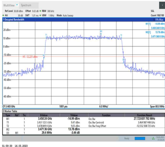
1-N78-3450-3550-PC1-30-30-L-8-CP-64QAM-Outer_Full-78@0-Ant0-27.724-29.400-≤30-PASS
