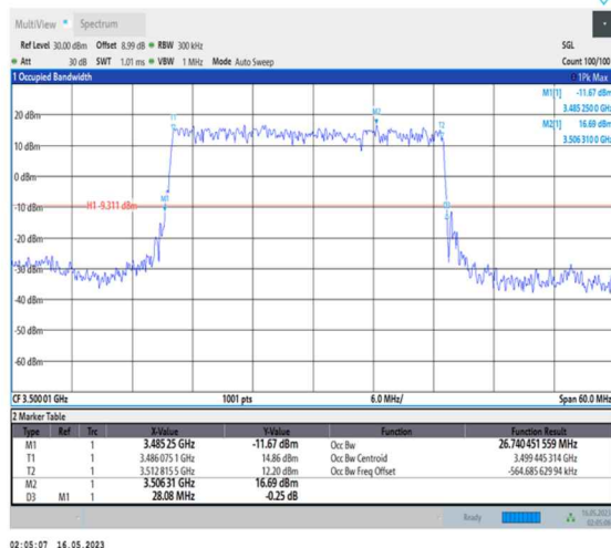
1-N78-3450-3550-PC1-30-30-M-2-DFT-Pi2BPSK-Outer_Full-75@0-Ant0-26.74-28.080-≤30-PASS
