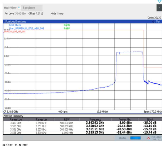
1-N78-3450-3550--30-30-H-6-CP-QPSK-Outer_Full-78@0-Ant0-PASS-see graph
