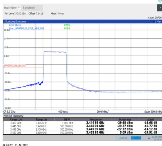
1-N78-3450-3550--30-30-L-6-CP-QPSK-Outer_Full-78@0-Ant0-PASS-see graph
