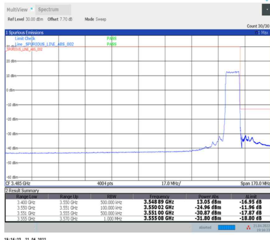
1-N78-3450-3550--30-10-H-3-DFT-PI2BPSK-Outer_Full-24@0-Ant0-PASS-see graph
