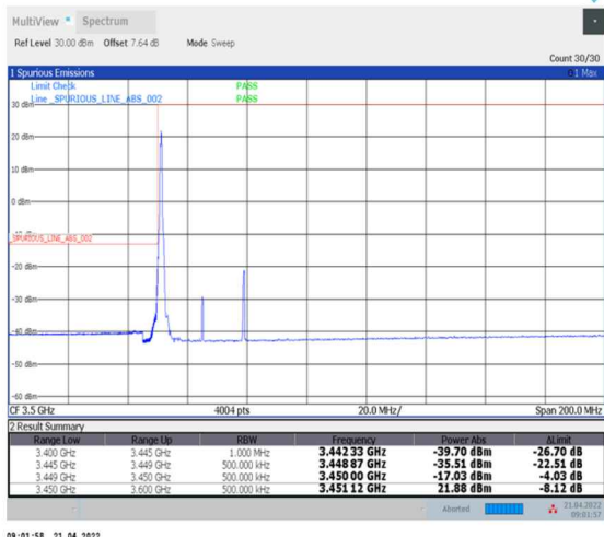
1-N78-3450-3550--30-30-L-1-DFT-PI2BPSK-Edge_1RB_Left-1@0-Ant0-PASS-see graph
