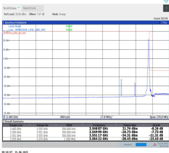
1-N78-3450-3550--30-30-H-5-CP-QPSK-Edge_1RB_Right-1@77-Ant0-PASS-see graph
