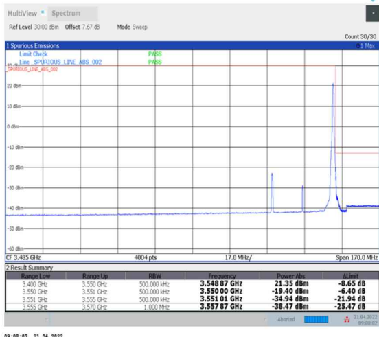
1-N78-3450-3550--30-30-H-2-DFT-PI2BPSK-Edge_1RB_Right-1@77-Ant0-PASS-see graph
