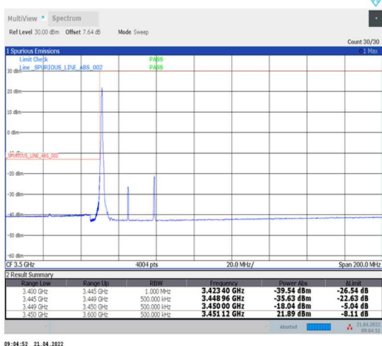
1-N78-3450-3550--30-30-L-4-CP-QPSK-Edge_1RB_Left-1@0-Ant0-PASS-see graph
