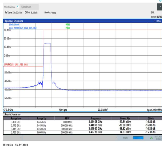
1-N78-3450-3550-PC1-30-10-L-3-DFT-PI2BPSK-Outer_Full-24@0-Ant0-1--PASS-see graph
