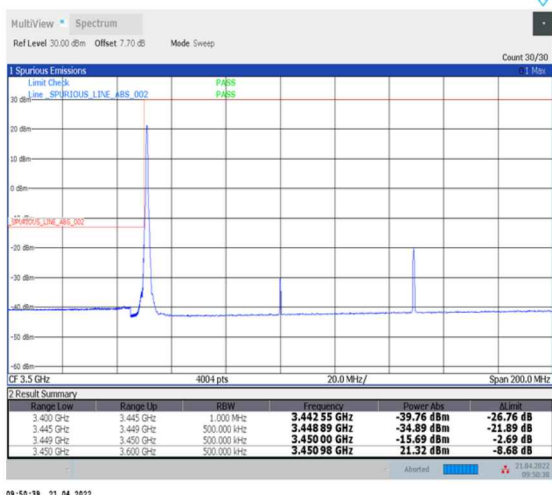
1-N78-3450-3550--30-100-L-1-DFT-PI2BPSK-Edge_1RB_Left-1@0-Ant0-PASS-see graph
