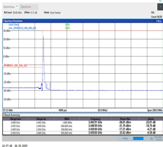
1-N78-3450-3550-PC1-30-10-L-4-CP-QPSK-Edge_1RB_Left-1@0-Ant0-1--PASS-see graph
