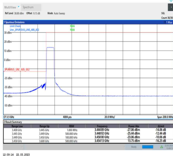
1-N78-3450-3550-PC1-30-10-L-6-CP-QPSK-Outer_Full-24@0-Ant0-1--PASS-see graph
