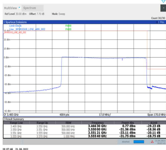
1-N78-3450-3550--30-90-H-6-CP-QPSK-Outer_Full-245@0-Ant0-PASS-see graph
