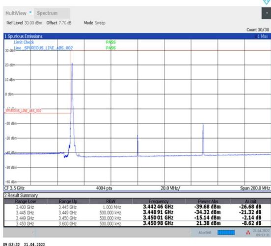
1-N78-3450-3550--30-100-L-4-CP-QPSK-Edge_1RB_Left-1@0-Ant0-PASS-see graph
