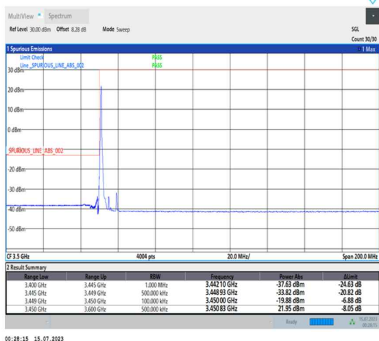
1-N78-3450-3550-PC1-30-10-L-1-DFT-PI2BPSK-Edge_1RB_Left-1@0-Ant0-1--PASS-see graph
