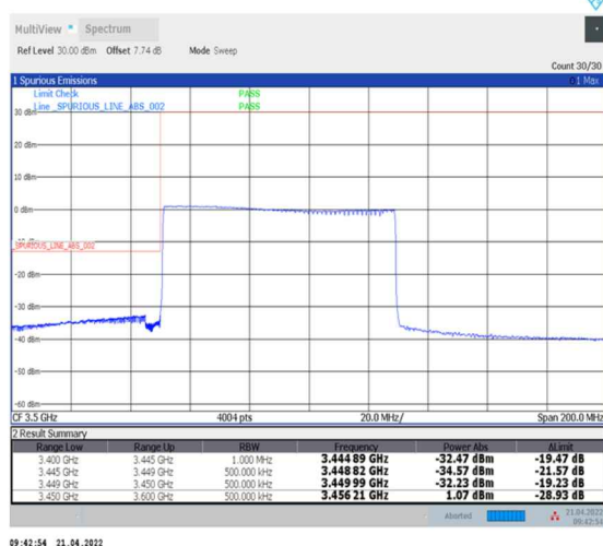
1-N78-3450-3550--30-80-L-6-CP-QPSK-Outer_Full-217@0-Ant0-PASS-see graph
