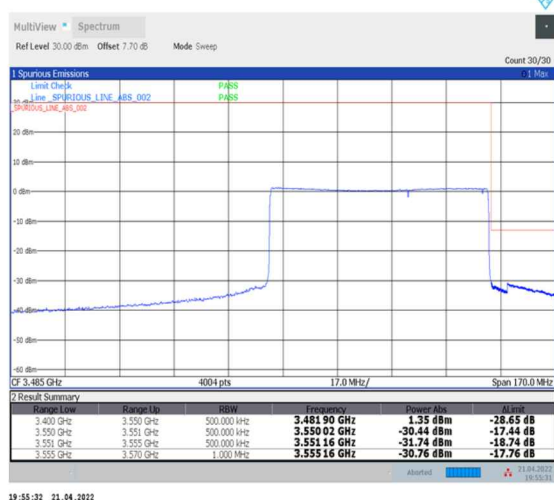
1-N78-3450-3550--30-70-H-6-CP-QPSK-Outer_Full-189@0-Ant0-PASS-see graph
