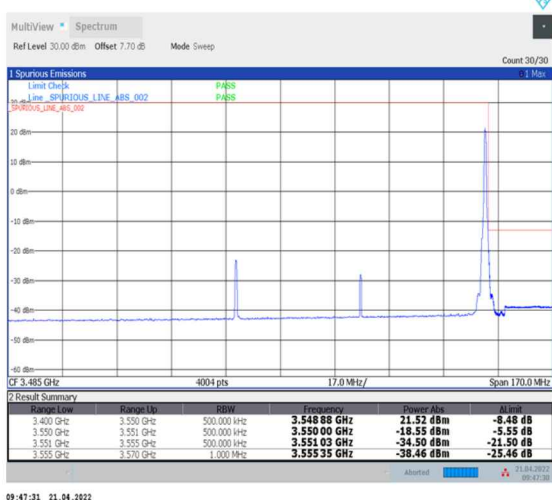
1-N78-3450-3550--30-80-H-5-CP-QPSK-Edge_1RB_Right-1@216-Ant0-PASS-see graph
