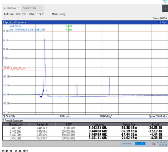
1-N78-3450-3550--30-80-L-4-CP-QPSK-Edge_1RB_Left-1@0-Ant0-PASS-see graph
