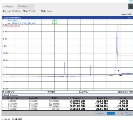
1-N78-3450-3550--30-70-H-5-CP-QPSK-Edge_1RB_Right-1@188-Ant0-PASS-see graph
