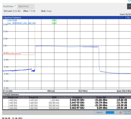
1-N78-3450-3550--30-100-L-6-CP-QPSK-Outer_Full-273@0-Ant0-PASS-see graph
