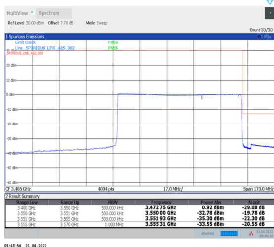
1-N78-3450-3550--30-80-H-6-CP-QPSK-Outer_Full-217@0-Ant0-PASS-see graph
