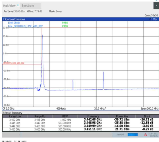
1-N78-3450-3550--30-80-L-1-DFT-PI2BPSK-Edge_1RB_Left-1@0-Ant0-PASS-see graph
