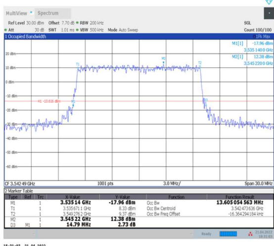
1-N78-3450-3550--30-15-H-6-CP-QPSK-Outer_Full-38@0-Ant0-13.605-14.790-≤15-PASS
