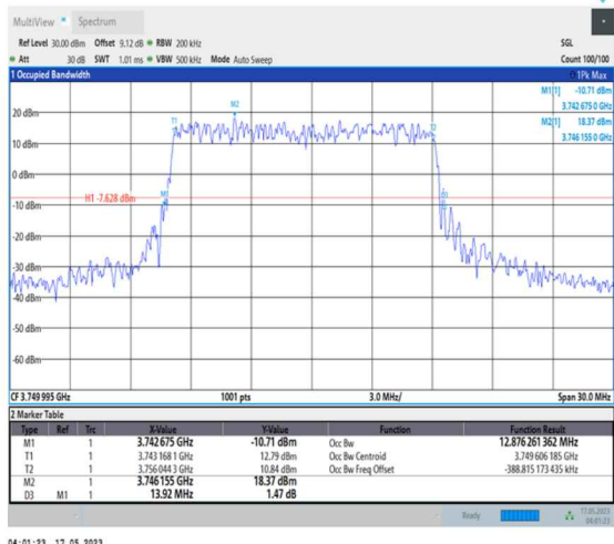
1-N78-3700-3800-PC1-30-15-M-1-DFT-QPSK-Outer_Full-36@0-Ant0-12.876-13.920-≤15-PASS
