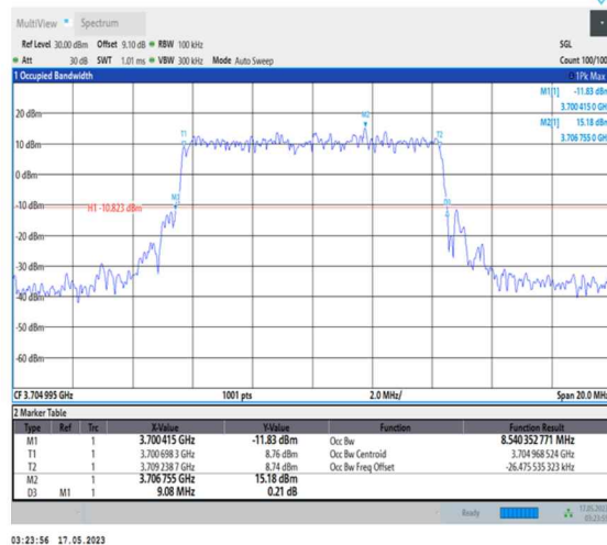
1-N78-3700-3800-PC1-30-10-L-4-DFT-64QAM-Outer_Full-24@0-Ant0-8.54-9.080-≤10-PASS
