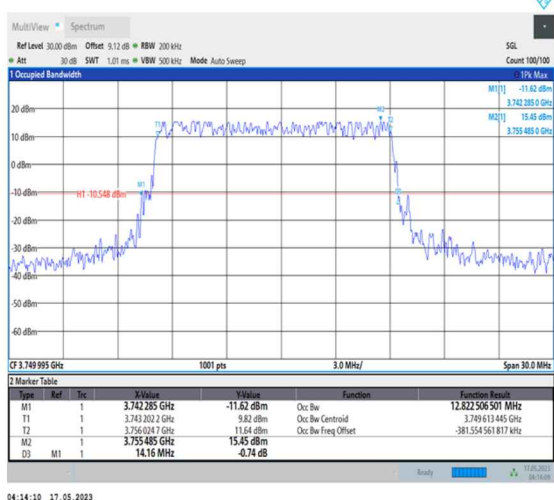
1-N78-3700-3800-PC1-30-15-M-3-DFT-16QAM-Outer_Full-36@0-Ant0-12.823-14.160-≤15-PASS
