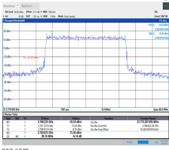
1-N78-3700-3800-PC1-30-40-H-7-CP-16QAM- Outer Full-106@0-Ant0-37.775-39.760-≤40-PASS
