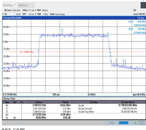
1-N78-3700-3800-PC1-30-40-H-9-CP-256QAM- Outer Full-106@0-Ant0-37.799-39.840-≤40-PASS
