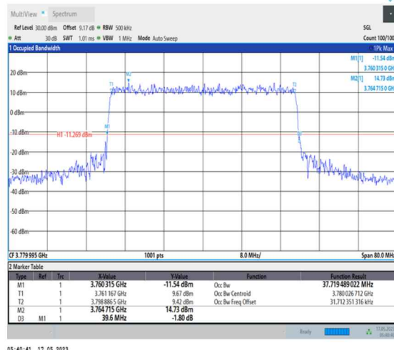
1-N78-3700-3800-PC1-30-40-H-8-CP-64QAM- Outer Full-106@0-Ant0-37.719-39.600-≤40-PASS
