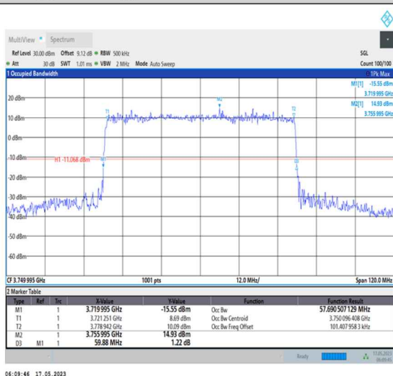
1-N78-3700-3800-PC1-30-60-M-4-DFT-64QAM- Outer Full-162@0-Ant0-57.691-59.880-≤60-PASS
