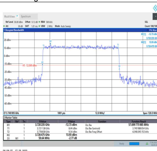
1-N78-3700-3800-PC1-30-60-M-3-DFT-16QAM- Outer Full-162@0-Ant0-57.7-59.640-≤60-PASS
