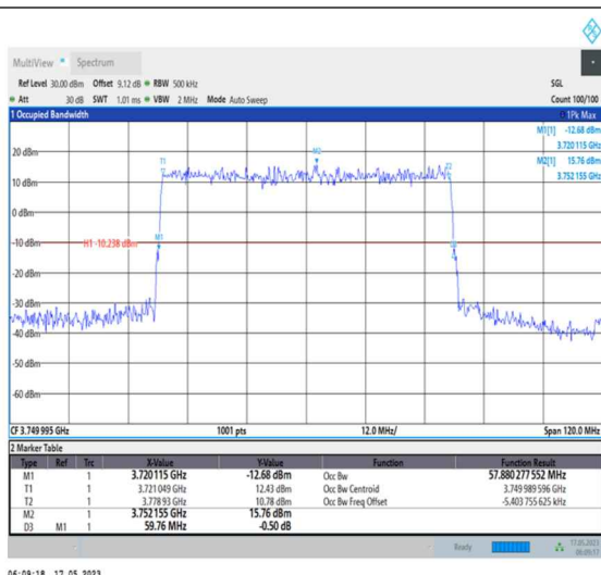
1-N78-3700-3800-PC1-30-60-M-2-DFT-PI2BPSK- Outer Full-162@0-Ant0-57.88-59.760-≤60-PASS
