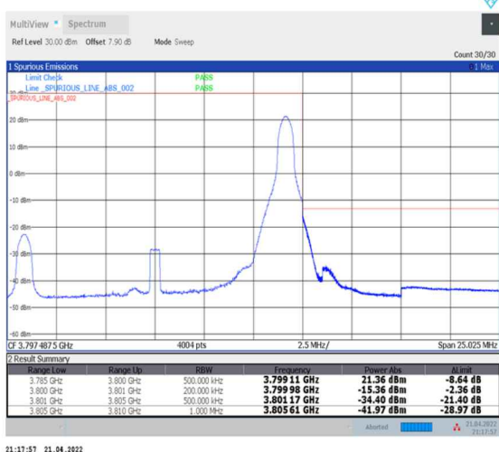
1-N78-3700-3800--30-15-H-5-CP-QPSK-Edge_1RB_Right-1@37-Ant0-PASS-see graph
