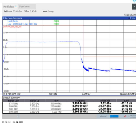
1-N78-3700-3800--30-15-H-6-CP-QPSK-Outer_Full-38@0-Ant0-PASS-see graph
