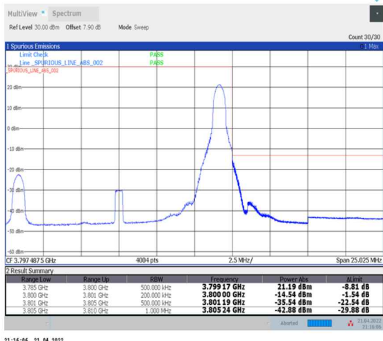
1-N78-3700-3800--30-15-H-2-DFT-PI2BPSK-Edge_1RB_Right-1@37-Ant0-PASS-see graph
