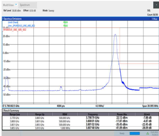
1-N78-3700-3800-PC1-30-30-H-2-DFT-PI2BPSK-Edge_1RB_Right-1@77-Ant0-1--PASS-see graph
