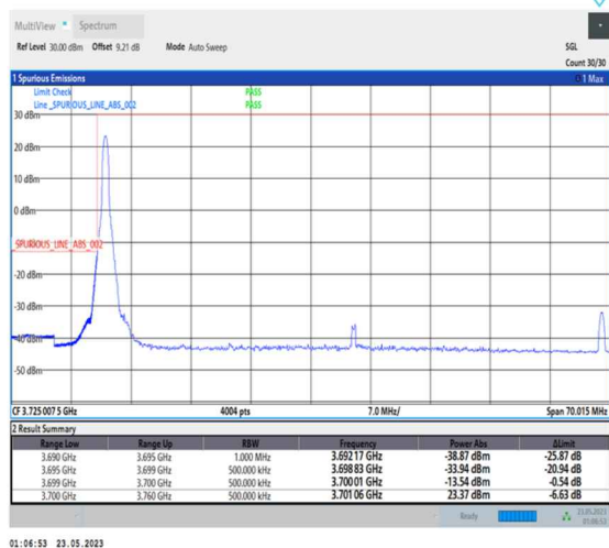
1-N78-3700-3800-PC1-30-60-L-4-CP-QPSK-Edge_1RB_Left-1@0-Ant0-1--PASS-see graph
