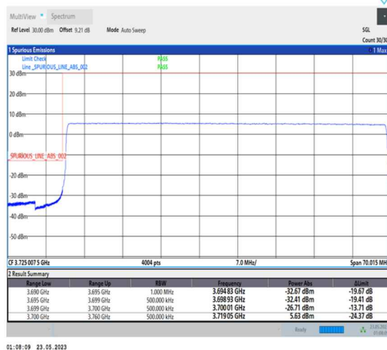
1-N78-3700-3800-PC1-30-60-L-6-CP-QPSK-Outer_Full-162@0-Ant0-1--PASS-see graph
