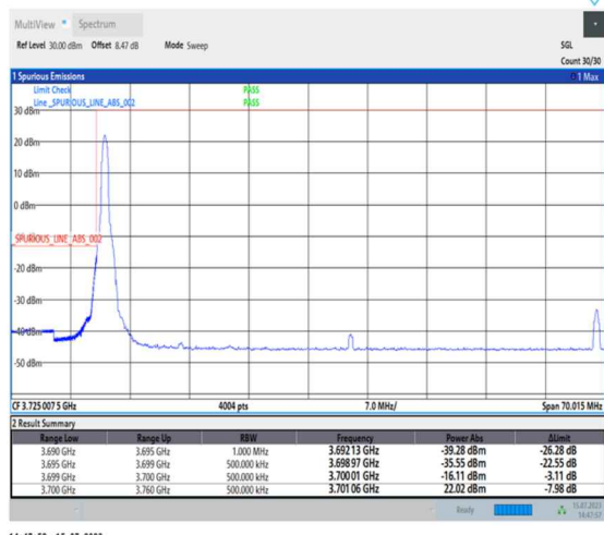
1-N78-3700-3800-PC1-30-60-L-1-DFT-PI2BPSK-Edge_1RB_Left-1@0-Ant0-1--PASS-see graph
