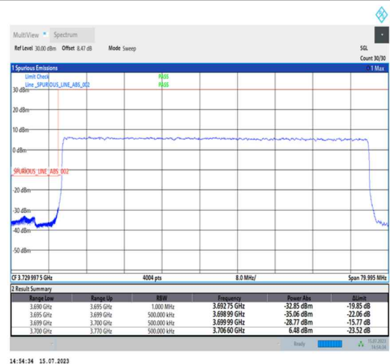
1-N78-3700-3800-PC1-30-70-L-3-DFT-PI2BPSK-Outer_Full-180@0-Ant0-1--PASS-see graph
