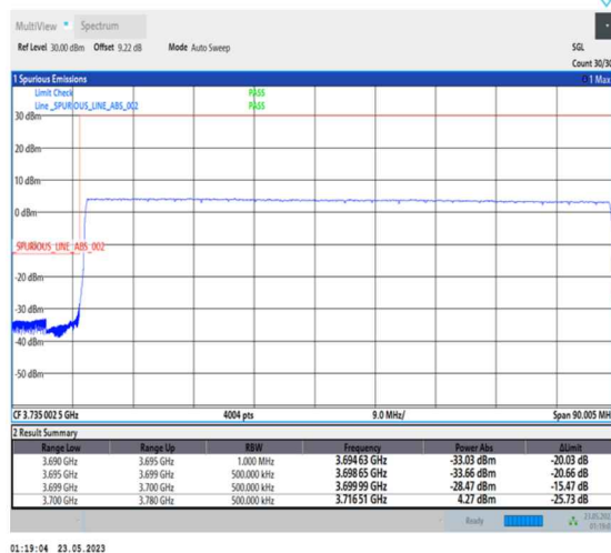
1-N78-3700-3800-PC1-30-80-L-6-CP-QPSK-Outer_Full-217@0-Ant0-1--PASS-see graph
