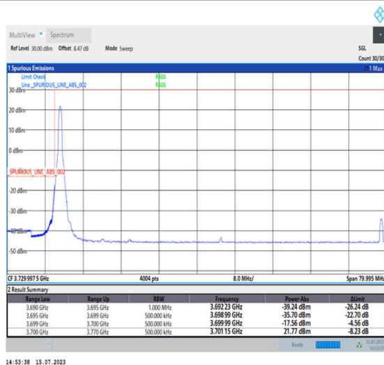
1-N78-3700-3800-PC1-30-70-L-1-DFT-PI2BPSK-Edge_1RB_Left-1@0-Ant0-1--PASS-see graph
