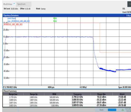
1-N78-3700-3800-PC1-30-30-H-3-DFT-PI2BPSK-Outer_Full-75@0-Ant0-1--PASS-see graph
