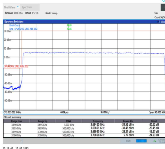
1-N78-3700-3800-PC1-30-80-L-3-DFT-PI2BPSK-Outer_Full-216@0-Ant0-1--PASS-see graph
