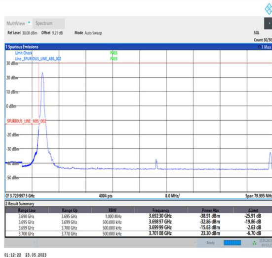
1-N78-3700-3800-PC1-30-70-L-4-CP-QPSK-Edge_1RB_Left-1@0-Ant0-1--PASS-see graph
