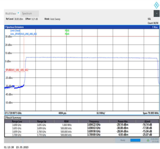
1-N78-3700-3800-PC1-30-70-L-6-CP-QPSK-Outer_Full-189@0-Ant0-1--PASS-see graph
