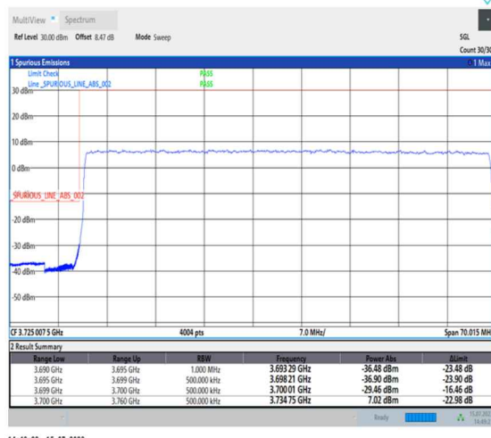
1-N78-3700-3800-PC1-30-60-L-3-DFT-PI2BPSK-Outer_Full-162@0-Ant0-1--PASS-see graph
