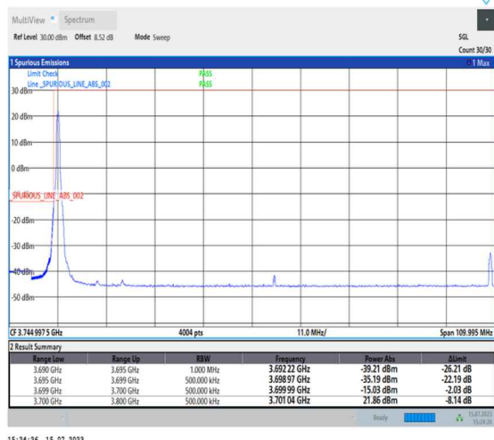
1-N78-3700-3800-PC1-30-100-L-1-DFT-PI2BPSK-Edge_1RB_Left-1@0-Ant0-1--PASS-see graph
