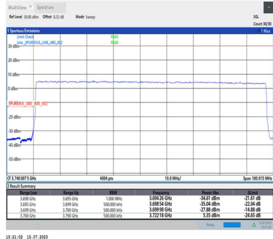
1-N78-3700-3800-PC1-30-90-L-3-DFT-PI2BPSK-Outer_Full-240@0-Ant0-1--PASS-see graph
