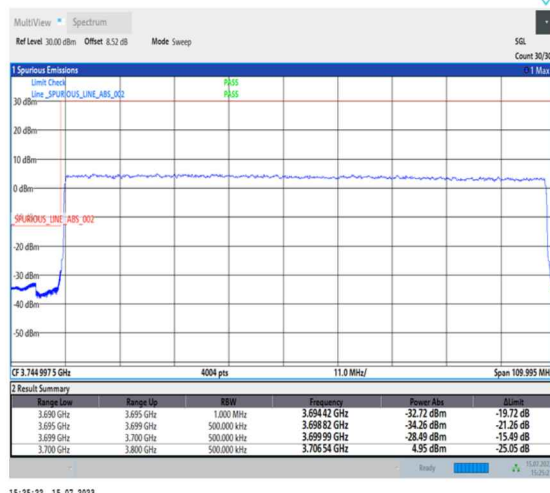
1-N78-3700-3800-PC1-30-100-L-3-DFT-PI2BPSK-Outer_Full-270@0-Ant0-1--PASS-see graph
