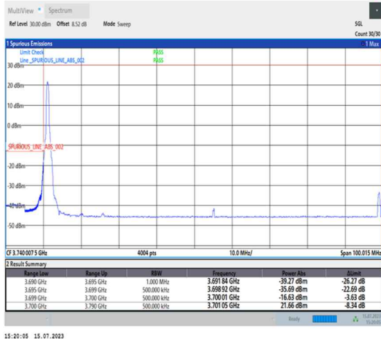
1-N78-3700-3800-PC1-30-90-L-1-DFT-PI2BPSK-Edge_1RB_Left-1@0-Ant0-1--PASS-see graph
