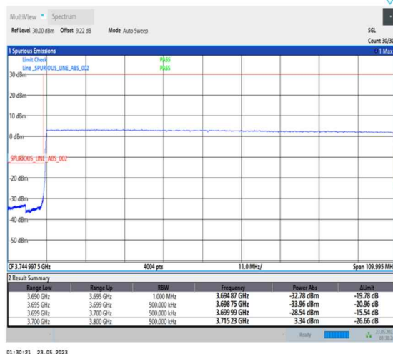
1-N78-3700-3800-PC1-30-100-L-6-CP-QPSK-Outer_Full-273@0-Ant0-1--PASS-see graph
