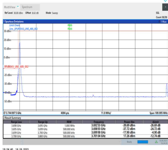
1-N78-3700-3800-PC1-30-100-L-4-CP-QPSK-Edge_1RB_Left-1@0-Ant0-1--PASS-see graph
