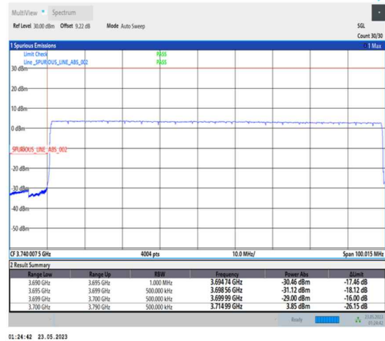
1-N78-3700-3800-PC1-30-90-L-6-CP-QPSK-Outer_Full-245@0-Ant0-1--PASS-see graph
