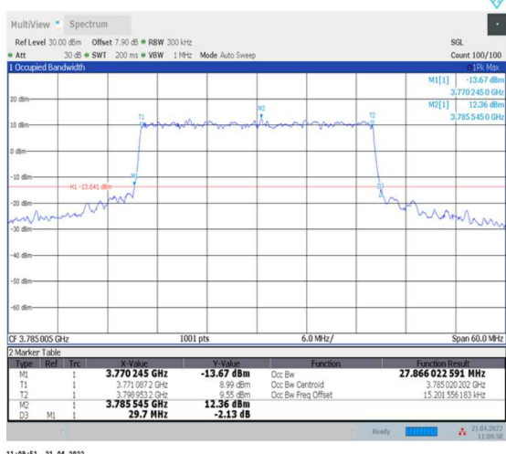
1-N78-3700-3800--30-30-H-8-CP-64QAM-Outer_Full-78@0-Ant0-27.866-29.700-≤30-PASS
