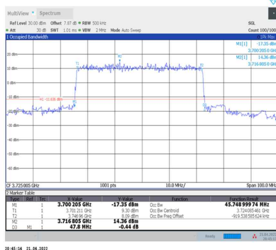
1-N78-3700-3800--30-50-L-1-DFT-QPSK-Outer_Full-128@0-Ant0-45.749-47.800-≤50-PASS
