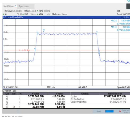
1-N78-3700-3800--30-30-H-9-CP-256QAM-Outer_Full-78@0-Ant0-27.847-29.880-≤30-PASS
