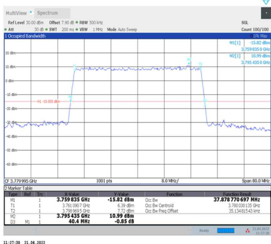
1-N78-3700-3800--30-40-H-9-CP-256QAM-Outer_Full-106@0-Ant0-37.879-40.400-≤40-PASS
