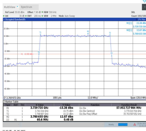
1-N78-3700-3800--30-60-H-4-DFT-64QAM-Outer_Full-162@0-Ant0-57.953-60.600-≤60-PASS
