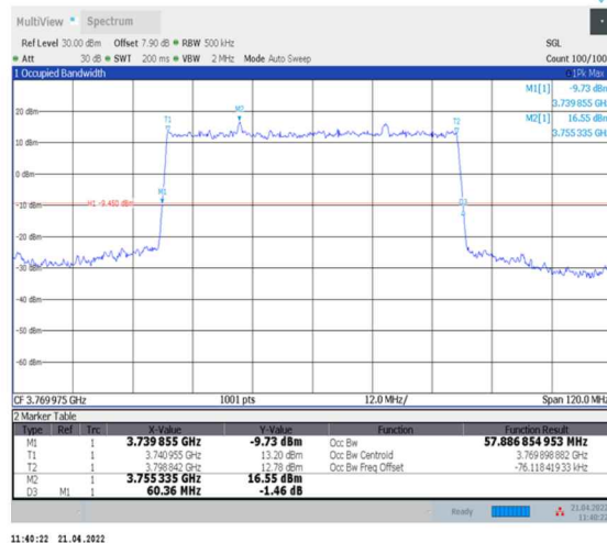
1-N78-3700-3800--30-60-H-2-DFT-PI2BPSK-Outer_Full-162@0-Ant0-57.887-60.360-≤60-PASS
