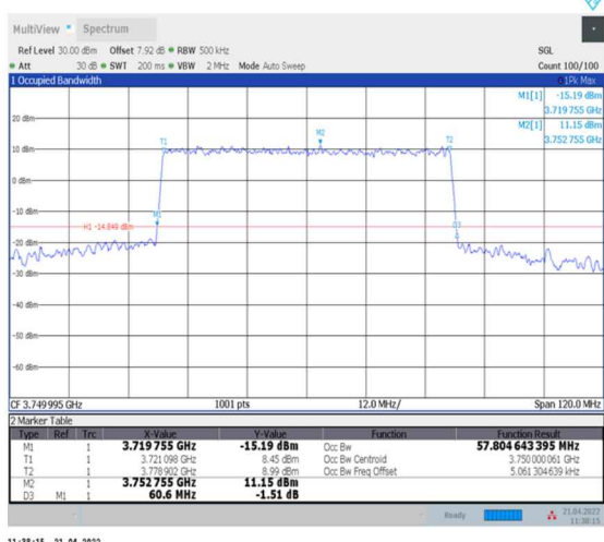
1-N78-3700-3800--30-60-M-8-CP-64QAM-Outter_Full-162@0-Ant0-57.805-60.600-≤60-PASS
