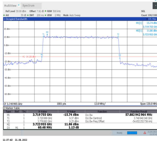
1-N78-3700-3800--30-60-M-7-CP-16QAM-Outter_Full-162@0-Ant0-57.883-60.480-≤60-PASS
