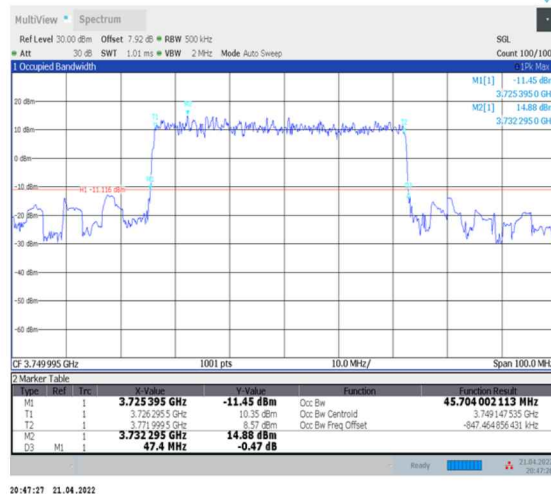
1-N78-3700-3800--30-50-M-2-DFT-PI2BPSK-Outer_Full-128@0-Ant0-45.704-47.400-≤50-PASS
