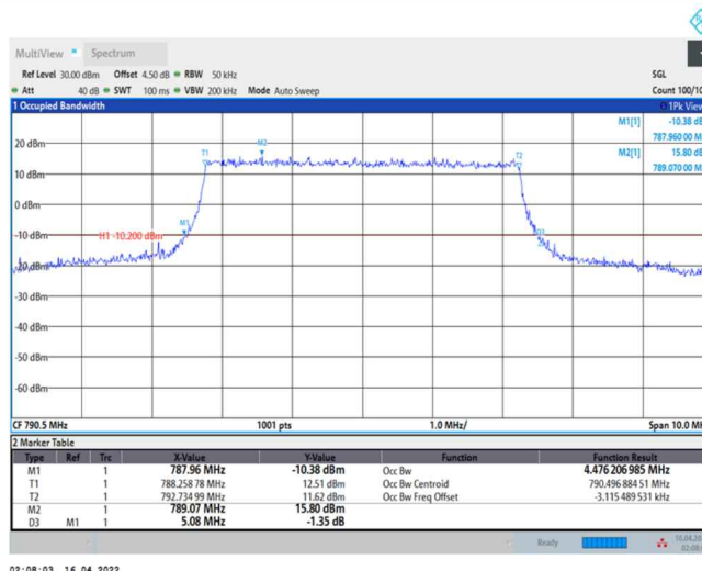
Band14-5MHz-QPSK-23330-25RB#0
