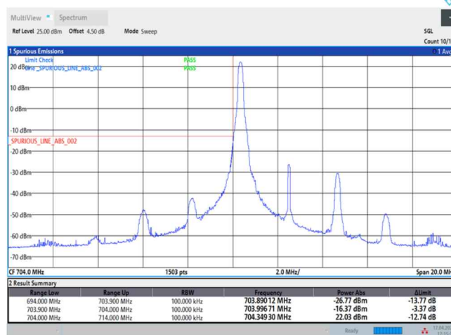
Band17-5MHz-QPSK-23755-25RB#0
