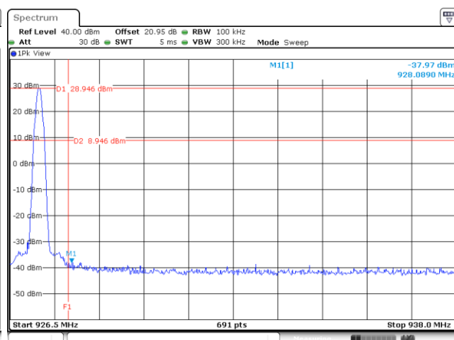
High Band Edge Plot on 927.25 MHz
