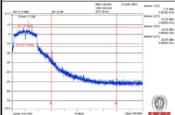
802.11n (20MHz) OFDM MODULATION (CH 116: 5580MHz)
