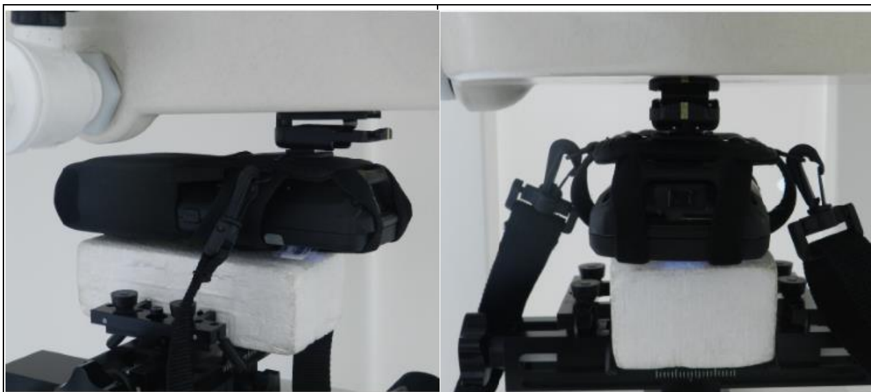
Back_0mm_Scanner 2_EUT Type 1_Holster 1
