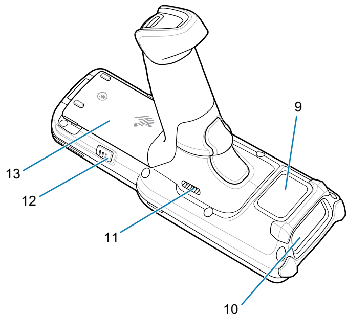
Figure 2 MC3300ax-G Back View
