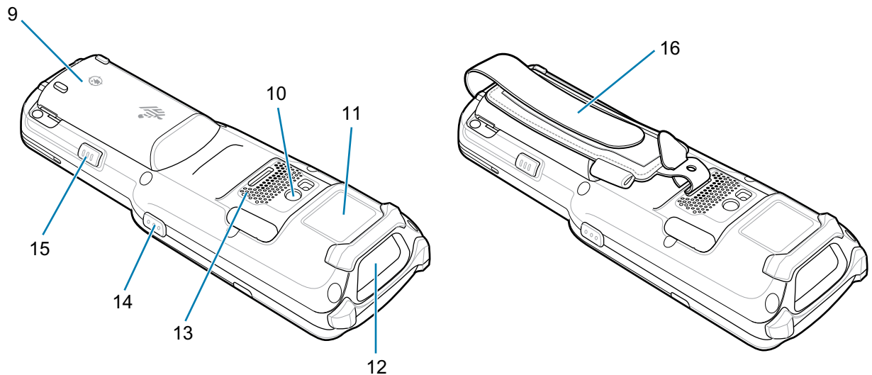
Figure 4 MC3300ax-S Back View
