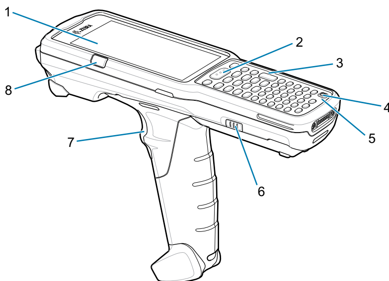
Figure 1 MC3300ax-G Front View
