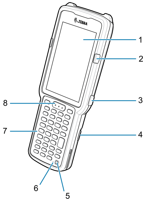
Figure 3 MC3300ax-S Front View
