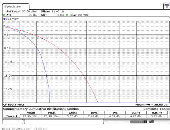
LTE Band 71 / 20MHz / 64QAM
