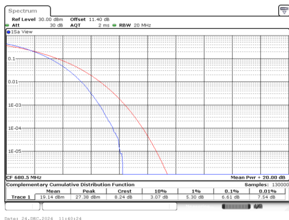
LTE Band 71 / 20MHz / 256QAM
