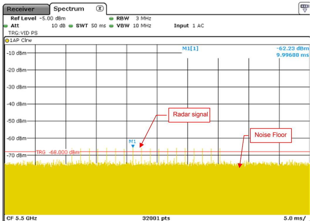
Radar Signal 0
