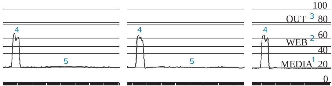
Figure 9 Media Sensor Profile (Black Mark Media)
