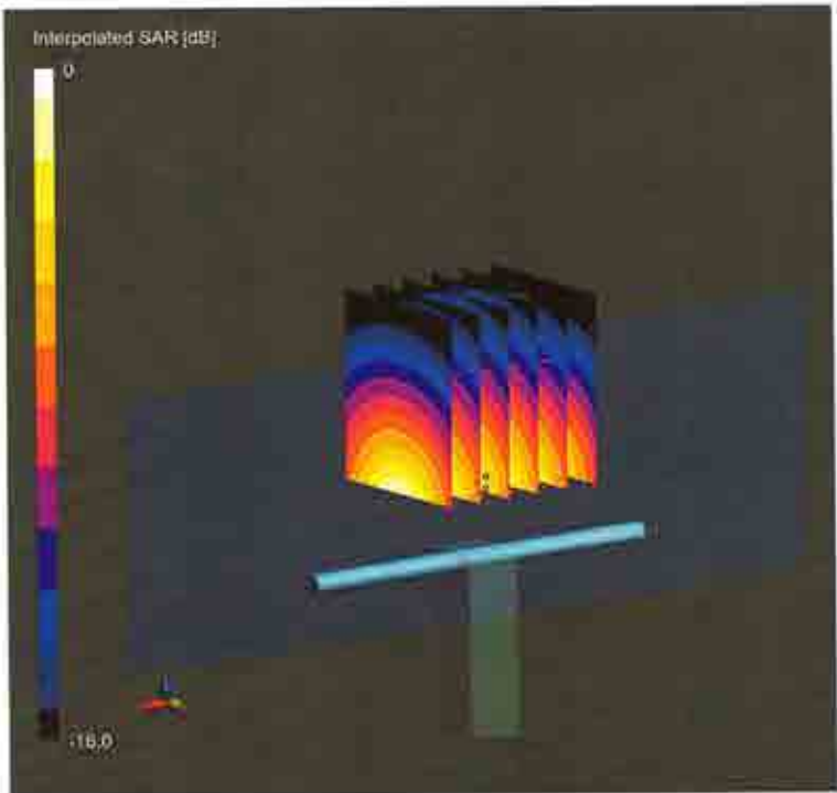
0 dB = 17.4 W/Kg
