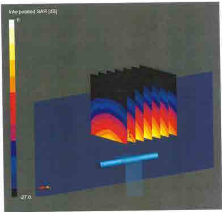
0 dB = 18.5 W/Kg
