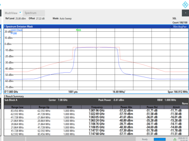
Plot on 7085 MHz
