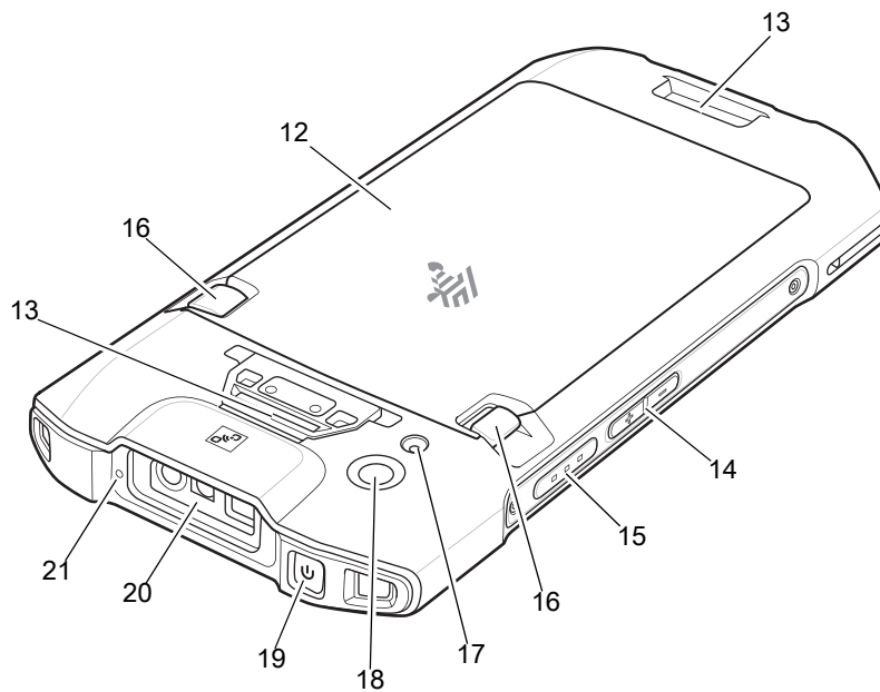
Figure 2 Rear View
