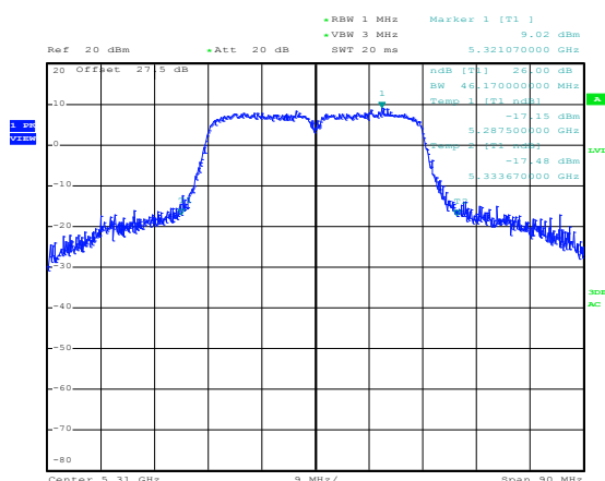
802.11a/n HT40 CH62 5310MHz
