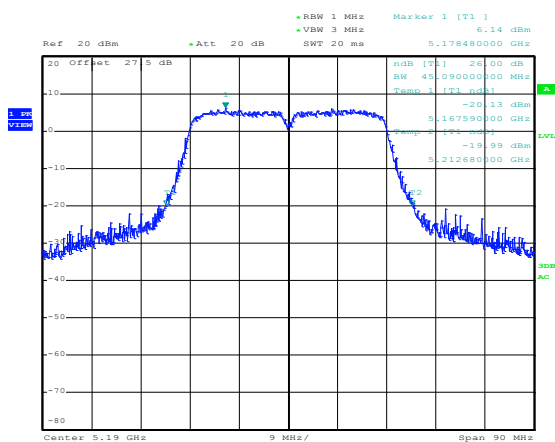
802.11a/n HT40 CH38 5190MHz
