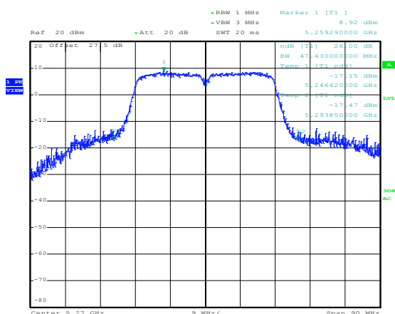
802.11a/n HT40 CH54 5270MHz
