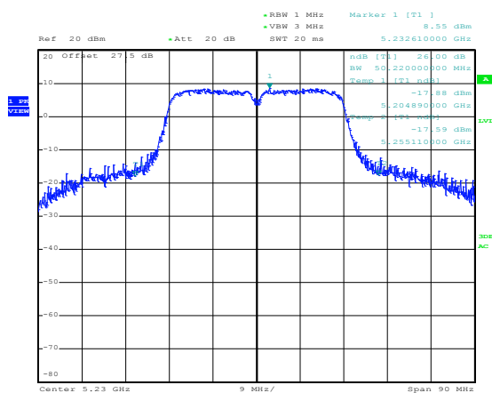
802.11a/n HT40 CH46 5230MHz
